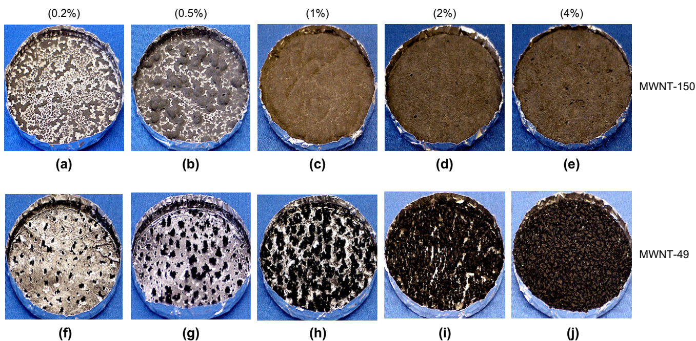
Fig. 10. Comparison of residues of PS/MWNT nanocomposites, based on MWNT-150 and MWNT-49, collected after the gasification test at 50 \text{ kW/m}^2 in nitrogen.
