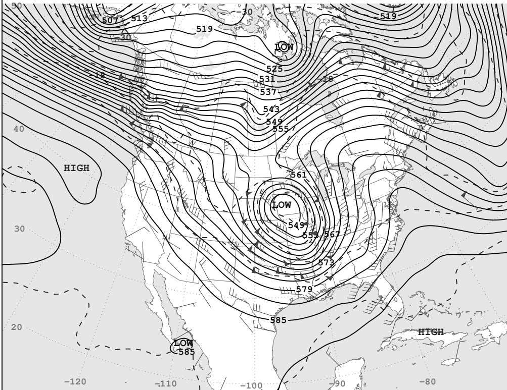
FRI, OCT 24, 2008 500-Millibar Height Contours at 7:00 A.M. E.S.T.
