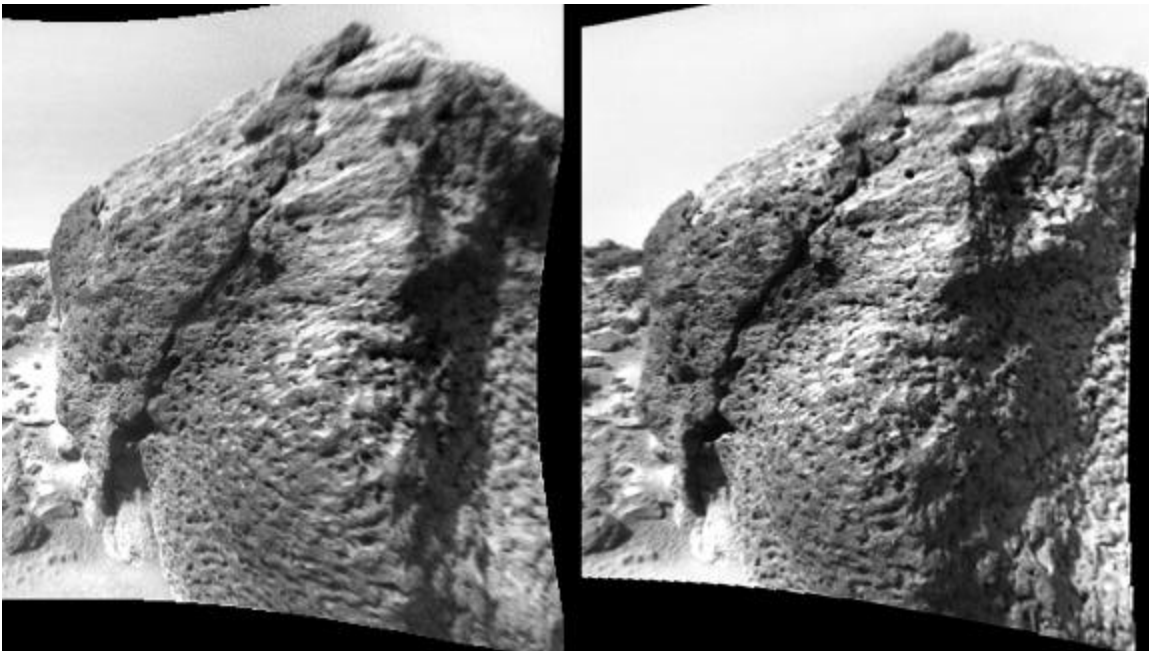
Figure 1: Rover forward camera stereo image of Chimp. Rock is 39 cm tall. Upper left texture resembles exfoliation. Prominent banding is roughly horizontal around the lower 2/3 of the rock, wrapping around the rounded nose closest to the camera, and continues around the left side of the rock.
