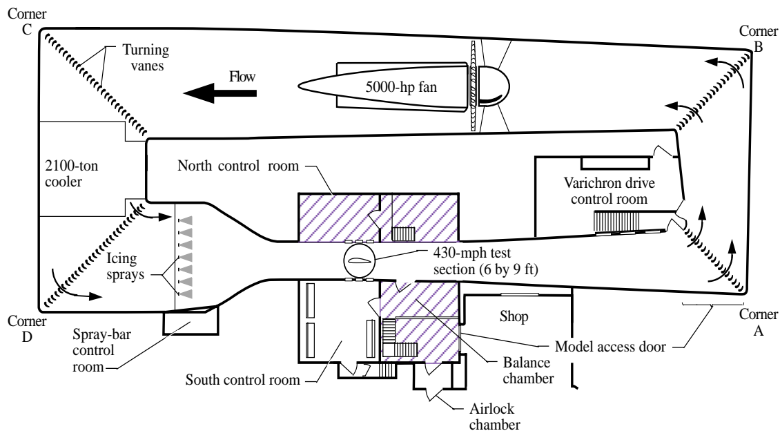
(a) Icing tunnel loop before rehabilitation.
