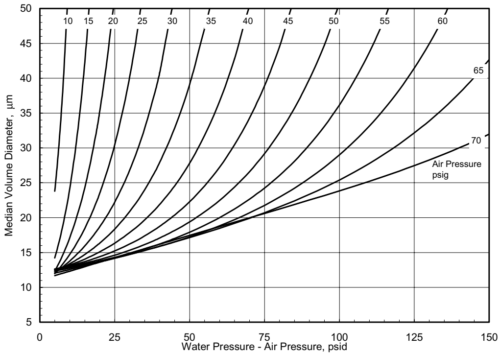
Figure 12.—The droplet size calibration curves for the Standard nozzles plotted as MVD versus \Delta P for the complete range of air pressures.
