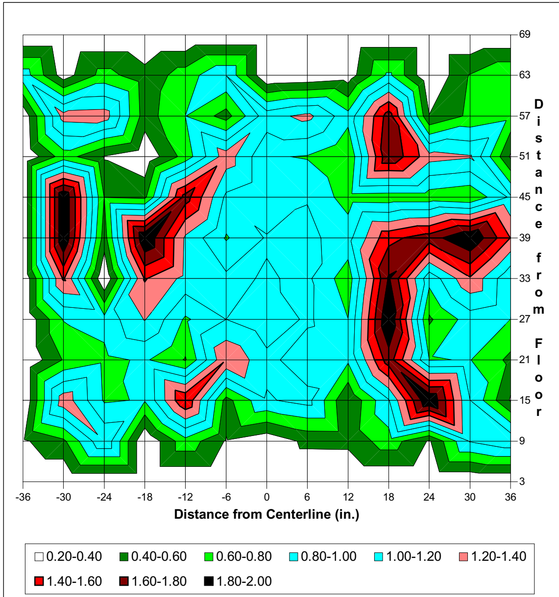
Figure 20.—The LWC uniformity contour plot for an MVD of 120 \mu\text{m} and an airspeed of 200 knots.
