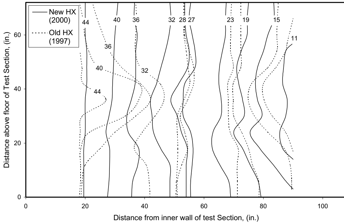
Figure 4.—Results from single columns of spray nozzles showing where the peak ice accretion occurs compared to a similar test with the previous heat exchanger.
