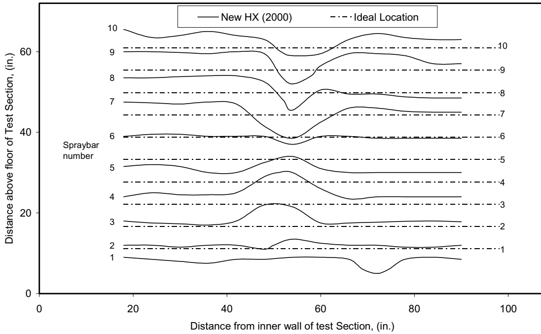
Figure 3.—Results from single spray bar test showing where the peak ice accretion occurs compared to the geometric projection of the spray bar locations into the test section.
