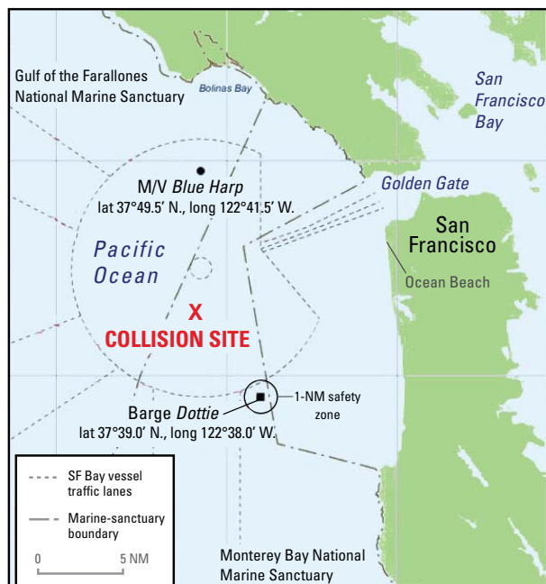
Golden Gate area, showing positions of the merchant vessel Blue Harp and the tank barge Dottie after a hypothetical collision 11 nautical miles southwest of the Golden Gate. Drift cards were released at these sites to simulate oil spilling from the damaged vessels and to test numerical models of ocean currents and oil-spill trajectories. NM, nautical mile. Modified from map at URL http://sanctuaries.noaa.gov/safeseas/images/exercisemap_large.jpg .
