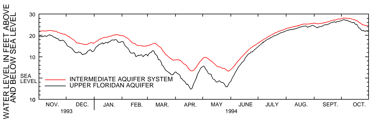
Figure 15. Seasonal flow measurements for Utopia No. 1 well in Sarasota County and hydrographs of the intermediate aquifer system and the Upper Floridan aquifer, November 1993 through October 1994.
