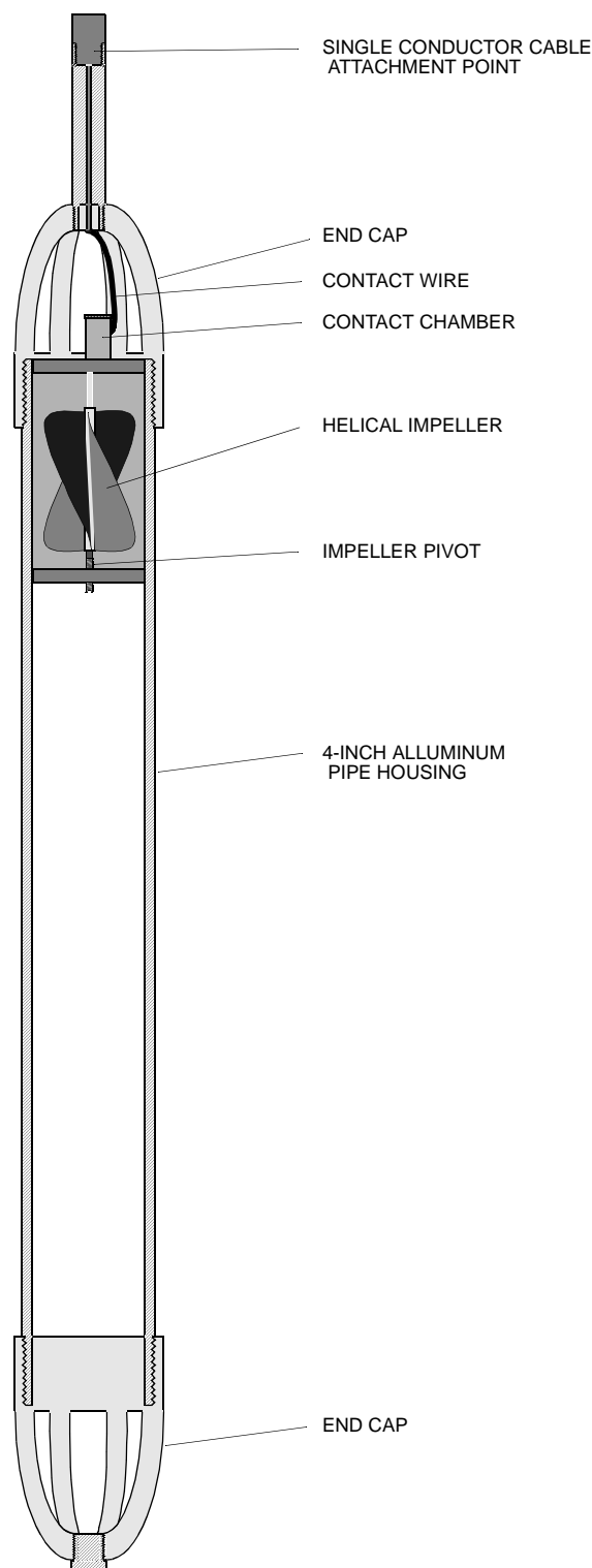
Figure 6. The components of the impeller flowmeter.
