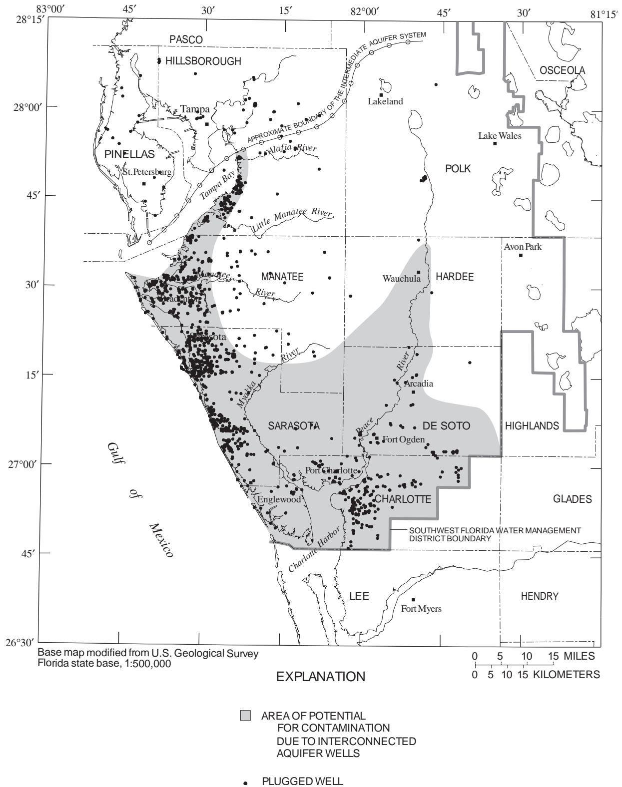
Figure 25. Area where there is a potential for water-quality degradation as a result of interconnected aquifers and locations of wells that have been plugged.
