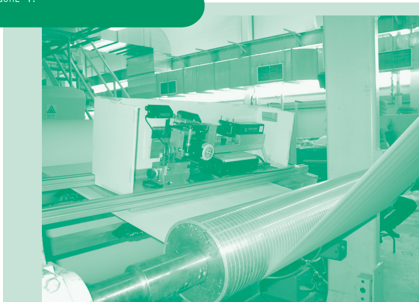
Partial view of the system for noncontact laser ultrasonic generation and detection on a moving paper web.
