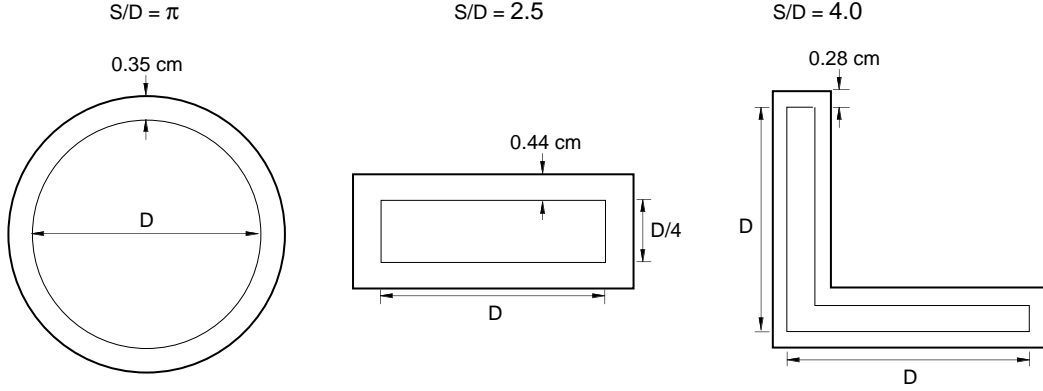
Figure 5. Equivalent uniform radial ice accretions on cylinders with circular, rectangular, and angle cross sections for a rainfall of 1 cm. The width of the rectangle is 1/4 of its length. The angle has equal-length legs with arbitrary thickness. The perimeter-to-“diameter” ratio S/D ranges from 3.14 for the circle to 2.5 for the rectangle and 4 for the angle.
