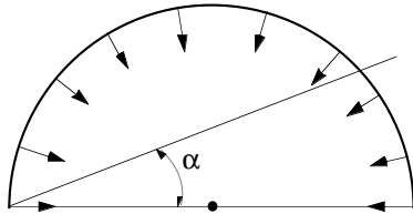
Figure B1. Sky diffuse solar radiation incident on surface inclined at an angle \alpha to the horizontal.
