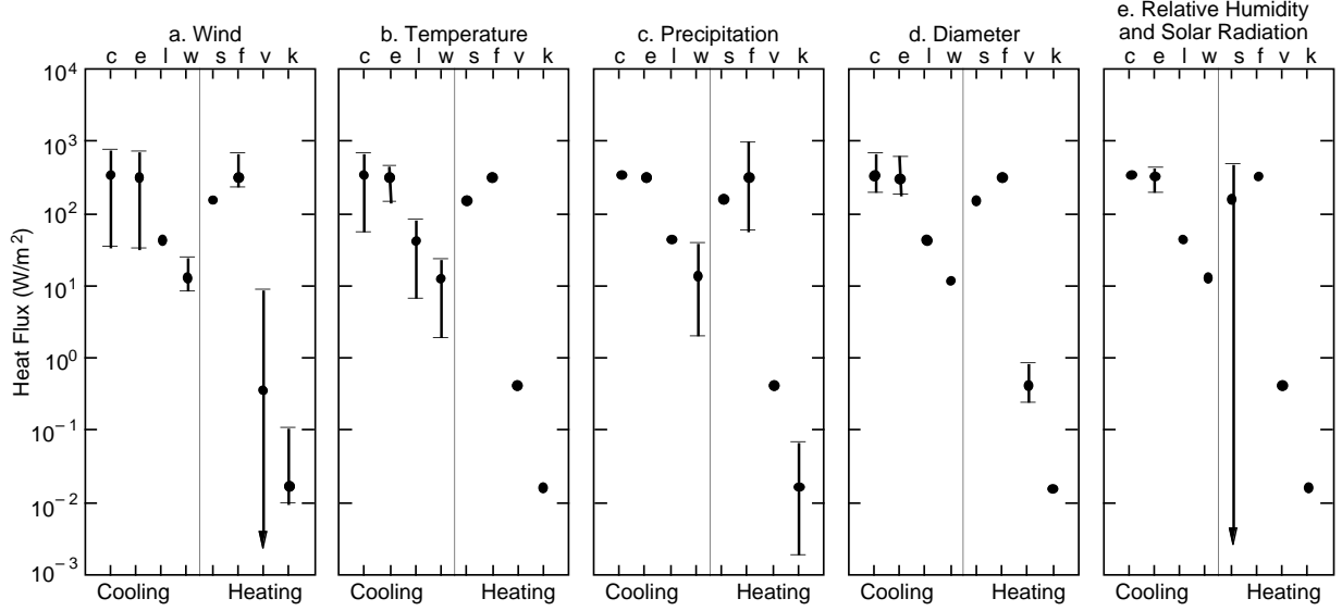
Figure 3. Comparison of heat flux terms in typical freezing-rain conditions. Standard conditions (black symbols) for the parameters are V = 3 m/s, T = -3^\circ\text{C} , P = 3 mm/hr, Rh = 0.90 , Sr = 100 W/m 2 , D_c = 3 cm. In each plot one or two of these parameters is varied about the standard conditions as follows: a) 0 < V < 10 m/s, b) -6 < T < -0.5^\circ\text{C} , c) 0.5 < P < 10 mm/hr, d) 0.5 < D_c < 10 cm, e) 0.80 < Rh < 1.00 and 0 < Sr < 200 W/m 2 . Minimum convective and evaporative fluxes in a) are provided by free convection. Key: e = evaporative cooling, c = convective cooling, l = longwave cooling, w = cooling from warming water, s = shortwave solar heating, f = heat of fusion, v = viscous heating, k = kinetic heating.
