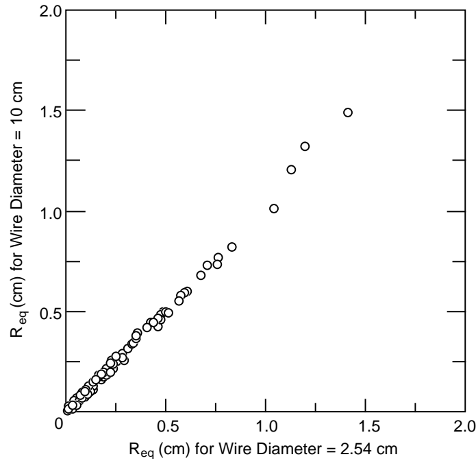
Figure 9. Comparison of uniform radial ice accretion thicknesses for 2.54- and 10-cm-diameter wires using the heat-balance model.
