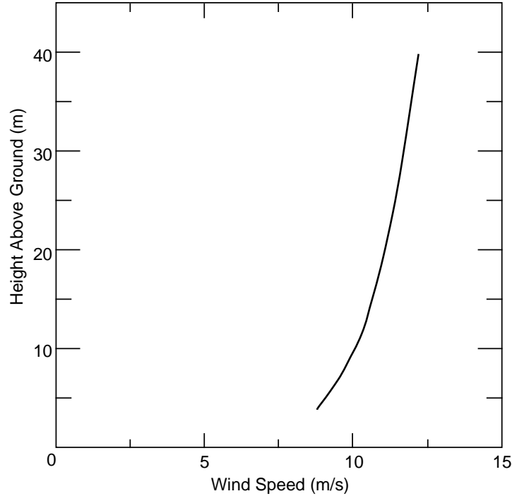
Figure 1. Wind profile for a 10-m/s wind at 10 m above ground assuming the 1/7 power law (ASCE 1994).
