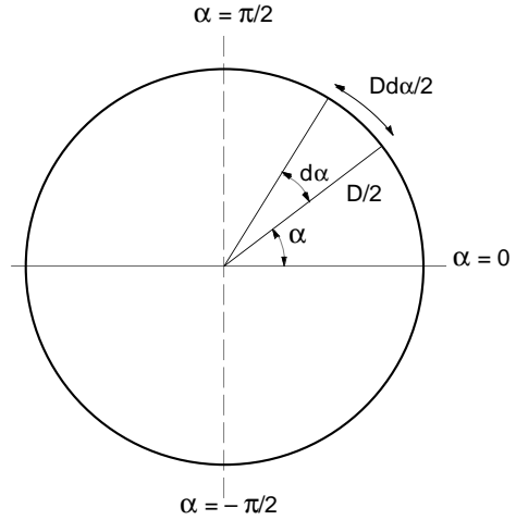
Figure B2. Cylinder surface elements.
