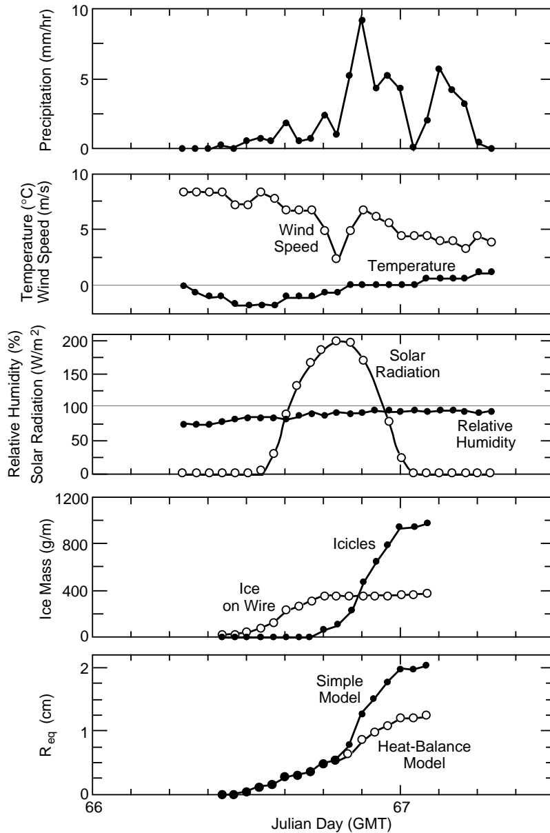
Figure 8. Time series of the weather conditions and hindcast ice accretions for the ice storm of 7–8 March 1990 at the Des Moines airport. The formation of icicles in the heat-balance model occurs in relatively warm, humid conditions. In those conditions the results from the heat-balance model and the simple flux model diverge.
