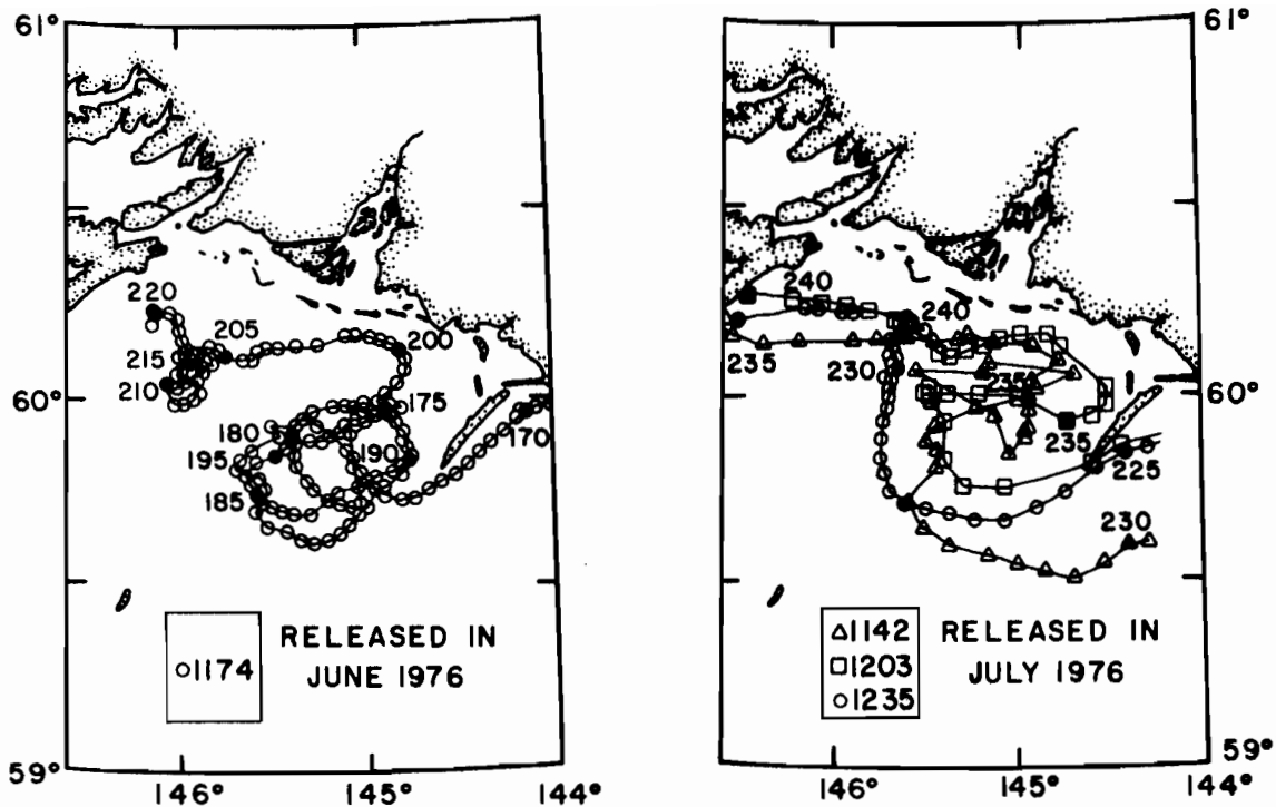
Figure 33. Satellite-tracked drifter trajectories west of Kayak Island in summer 1976.
