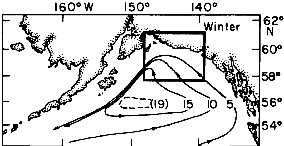
Figure 3. Schematic showing winter water transport in million cubic meters per second computed from wind stress curl (from Ingraham et al. , 1976). Rectangle shows our study region, approximately the area included in Figure 1.
