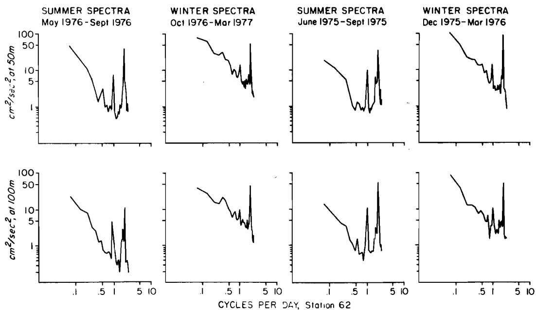
Figure 12. Kinetic energy spectra for winter and summer observations at two depths at station 62.
