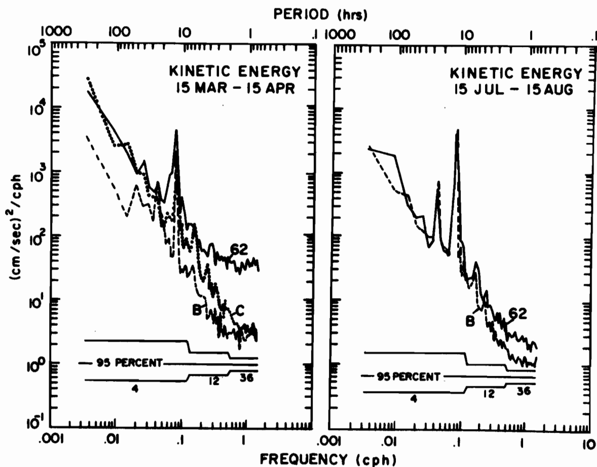
Figure 6. Comparison of the kinetic energy spectra at locations 62, B, and C in spring and at B and 62 in summer. Moorings B and C had upper flotation at 45 m, mooring 62 had flotation at 17 m.
