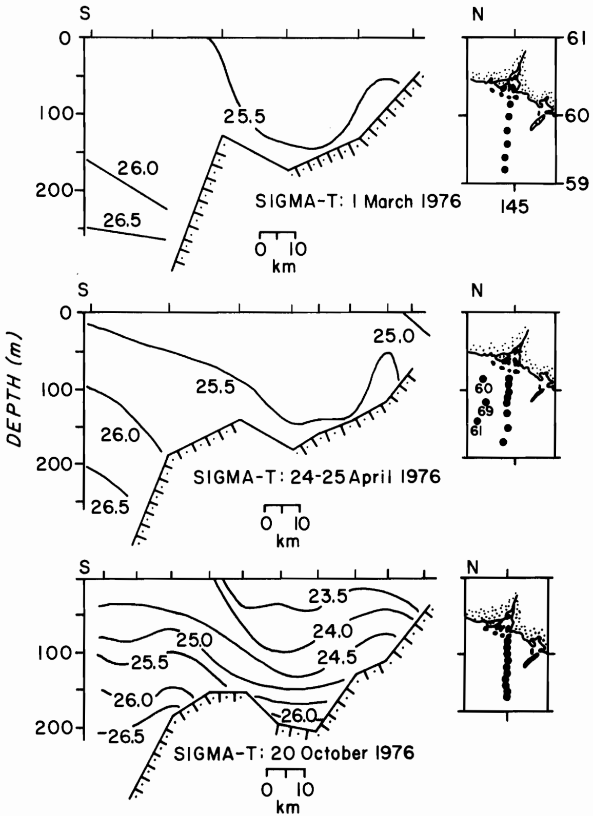
Figure 36. Vertical distribution of density (as \sigma_t ) west of Kayak Island for three periods in 1976.
