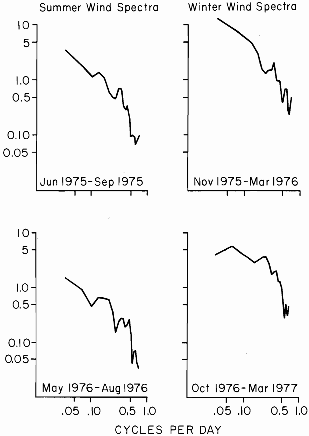
Figure 15. Kinetic energy spectra for geostrophic winds at station 62.
