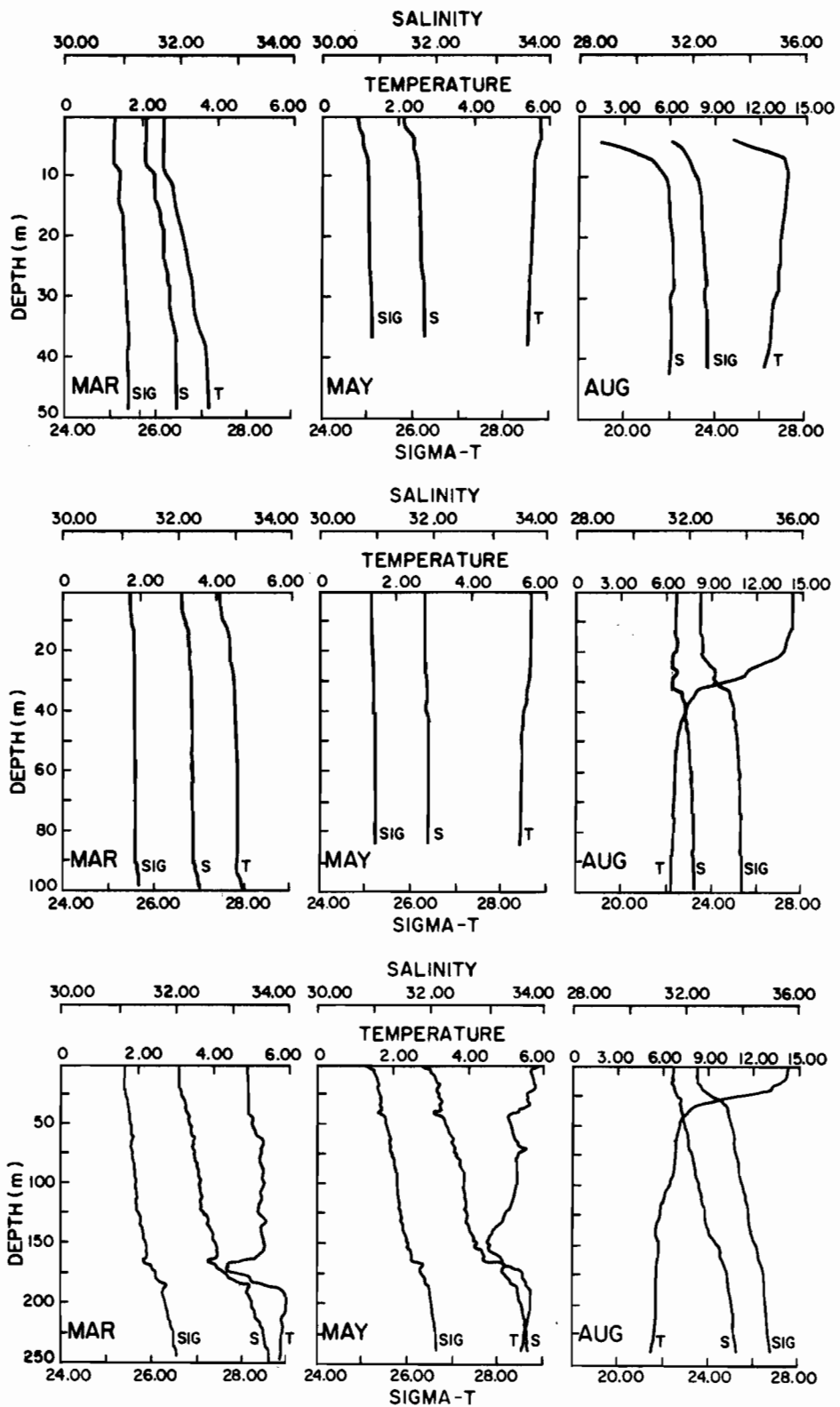
Figure 21. Seasonal variation of the temperature, salinity, and sigma-t profiles at the three depths where bottom pressure was measured.
