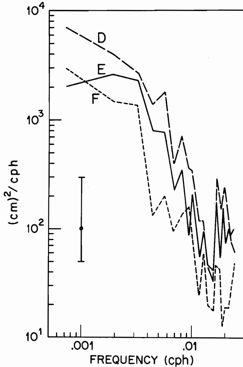
Figure 28. Spectra of bottom pressure records at sites D, E, and F. The error bars indicate 95 percent confidence interval.
