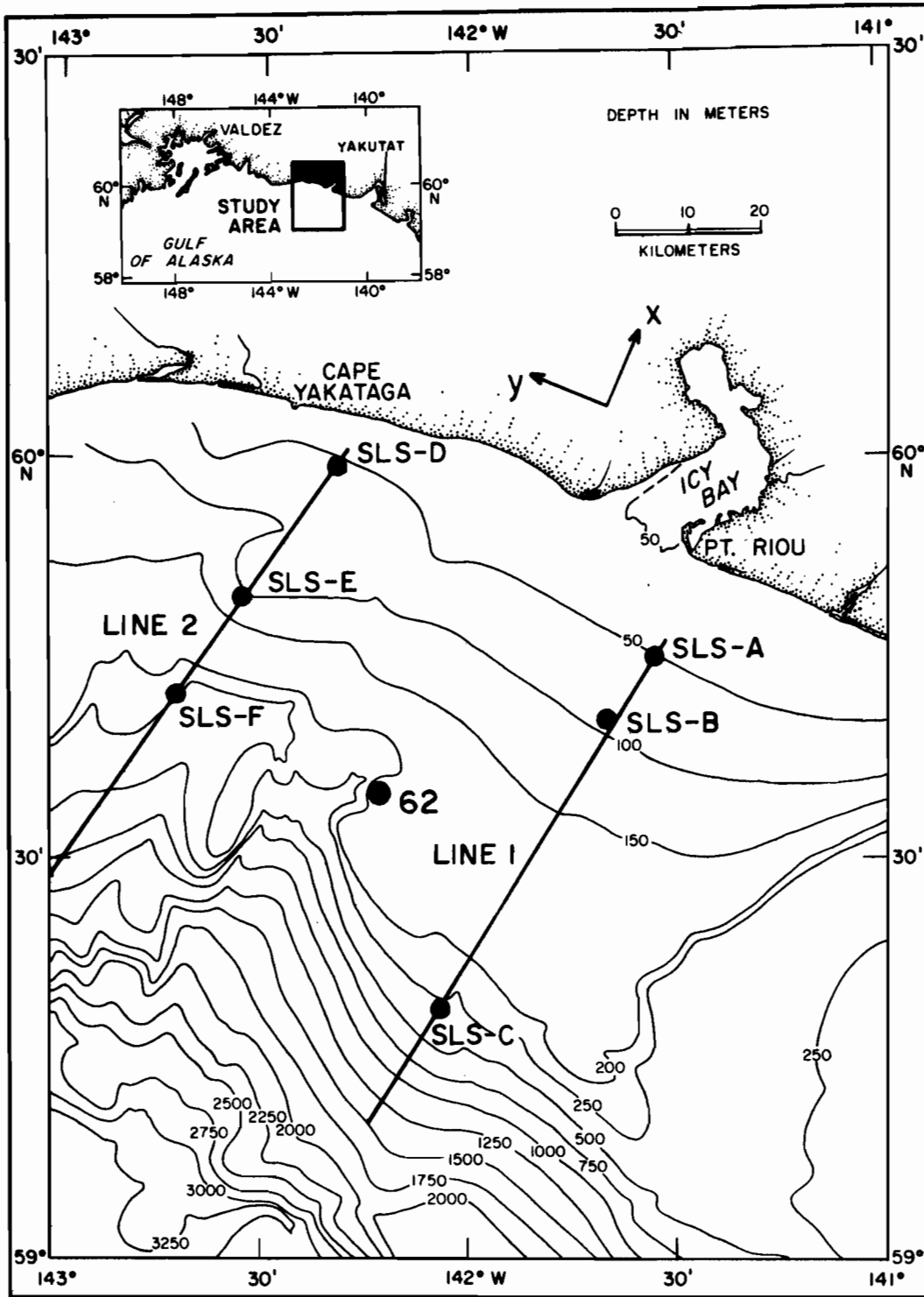
Figure 19. Location of the experiment off Icy Bay, Alaska. The coordinate system indicates the alongshore direction, y , and the cross-shelf direction, x .
