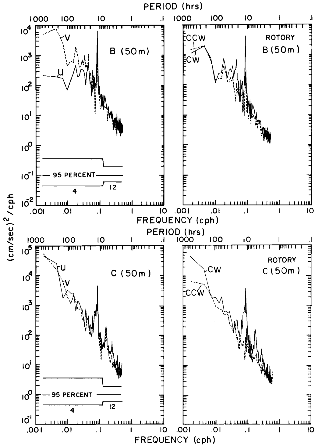
Figure 27. Rectilinear and rotary kinetic energy spectra at the 50-m depth at locations B and C.
