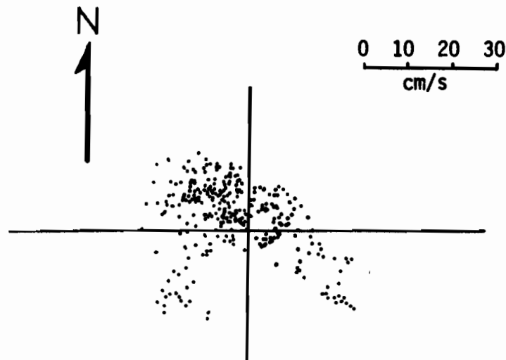
Figure 10. Progressive vector diagram and scatter plot for station 62 during summer.
