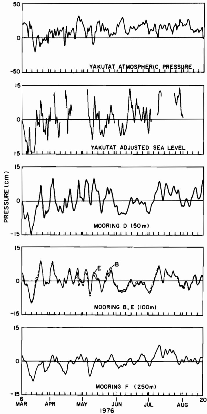
Figure 23. Time series of atmospheric pressure and adjusted sea level at Yakutat and of bottom pressure at B, D, E, and F. All records have been low-pass filtered. The gaps in adjusted sea level are caused by missing tide gage data. It is assumed that 1 cm = 1 mb.
