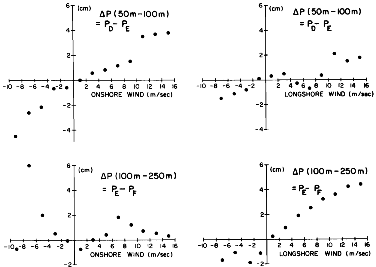
Figure 32. Cross-shelf pressure gradient between indicated depth contours vs. onshore and alongshore wind.
