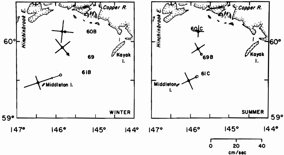
Figure 34. Arrows indicate mean current vectors, while cross-bars indicate variance, at three locations west of Kayak Island during winter and summer 1976.
