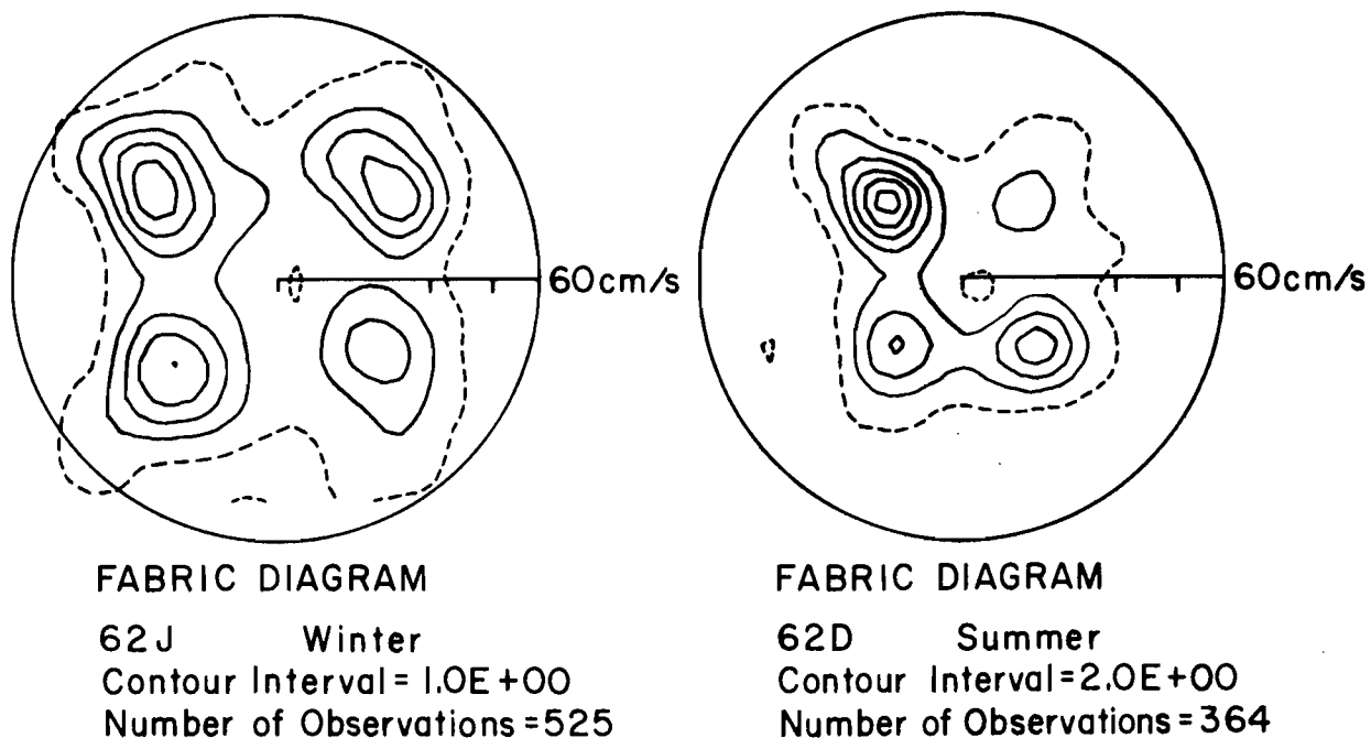
Figure 11. Fabric diagrams showing directional trends in representative winter and summer current records at station 62.
