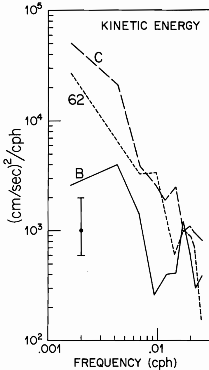
Figure 26. Kinetic energy spectra of the low-frequency fluctuation at B, C, and 62 for the period 15 March-15 May.
