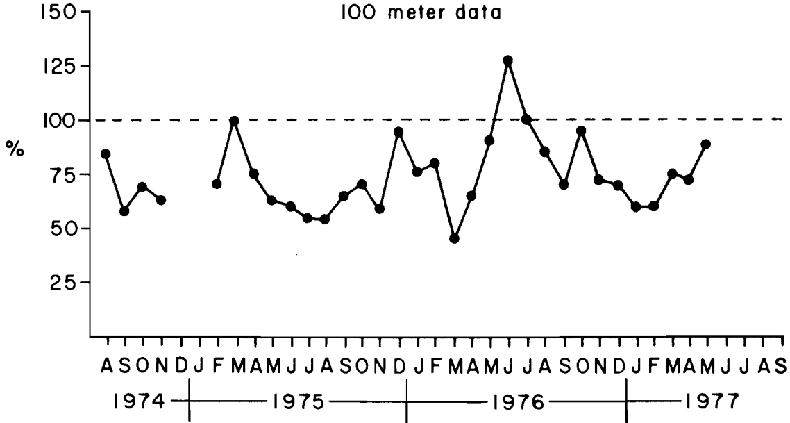
Figure 14. Standard deviation of currents as percent of average speed squared, plotted vs. time.
