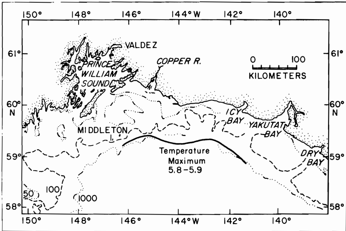
Figure 2. Axis of subsurface temperature maximum used as an indicator of flow streamlines in the Alaska Current in the northeast Gulf of Alaska (from Galt and Royer, in press).
