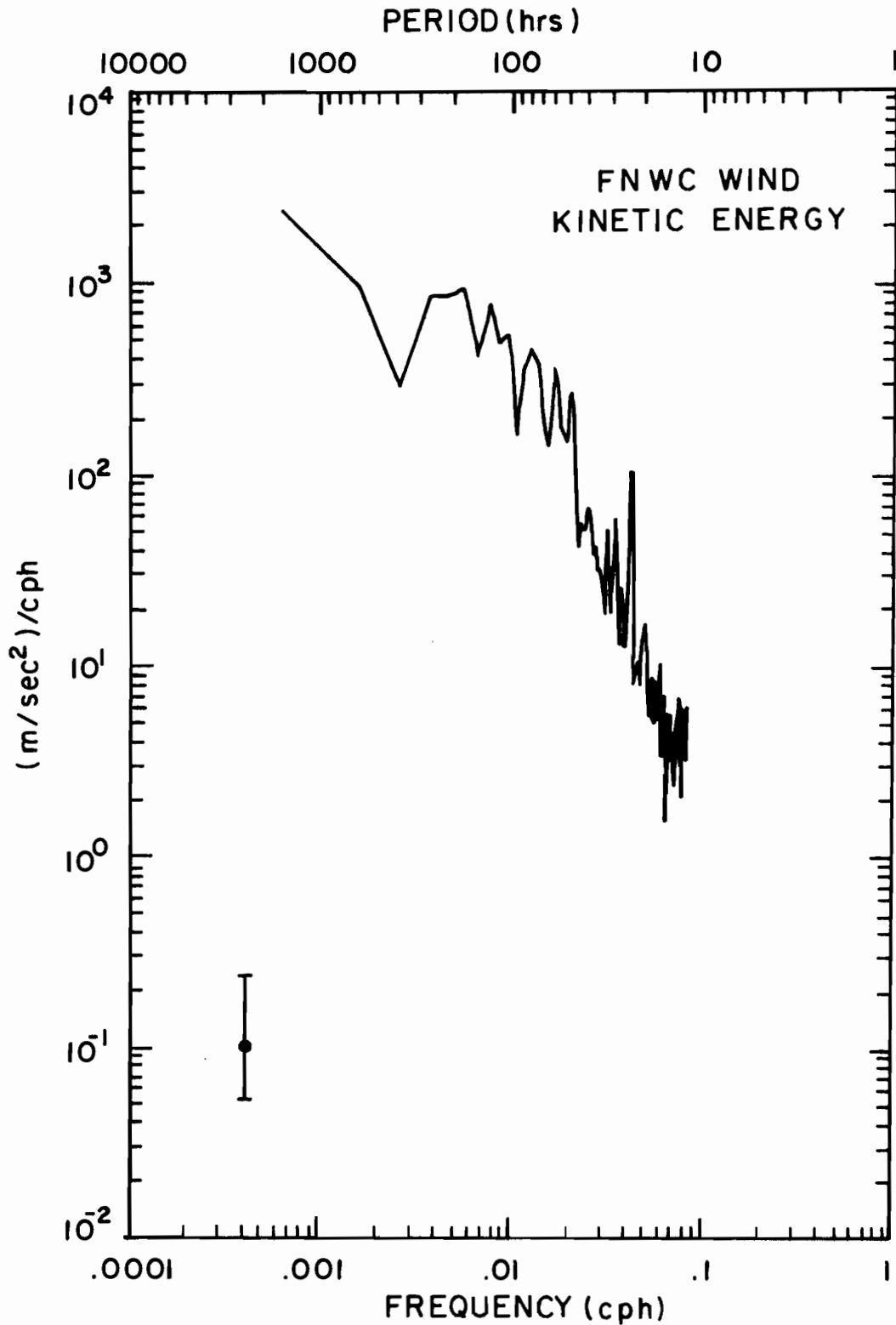
Figure 31. Kinetic energy spectrum of the FNWC wind. The error bars indicate 95 percent confidence interval.
