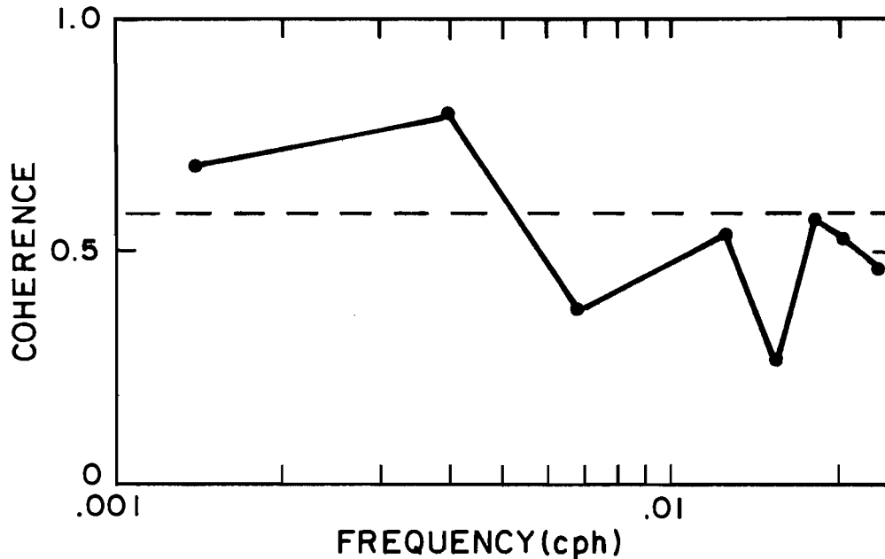
Figure 29. Coherence between bottom pressure measured at sites D (50-m depth) and F (250-m depth). The dashed line indicates the 95 percent confidence level for zero coherence.
