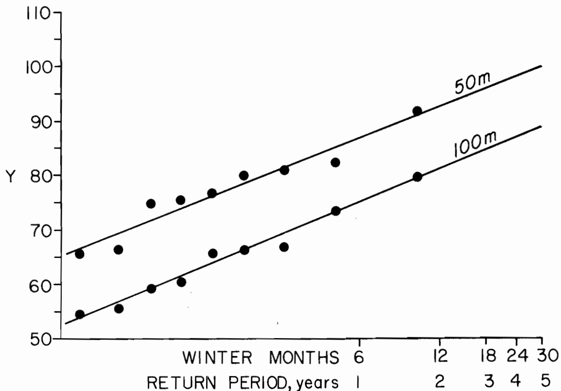
Figure 18. Plot of projected extreme values Y vs. time at station 62.
