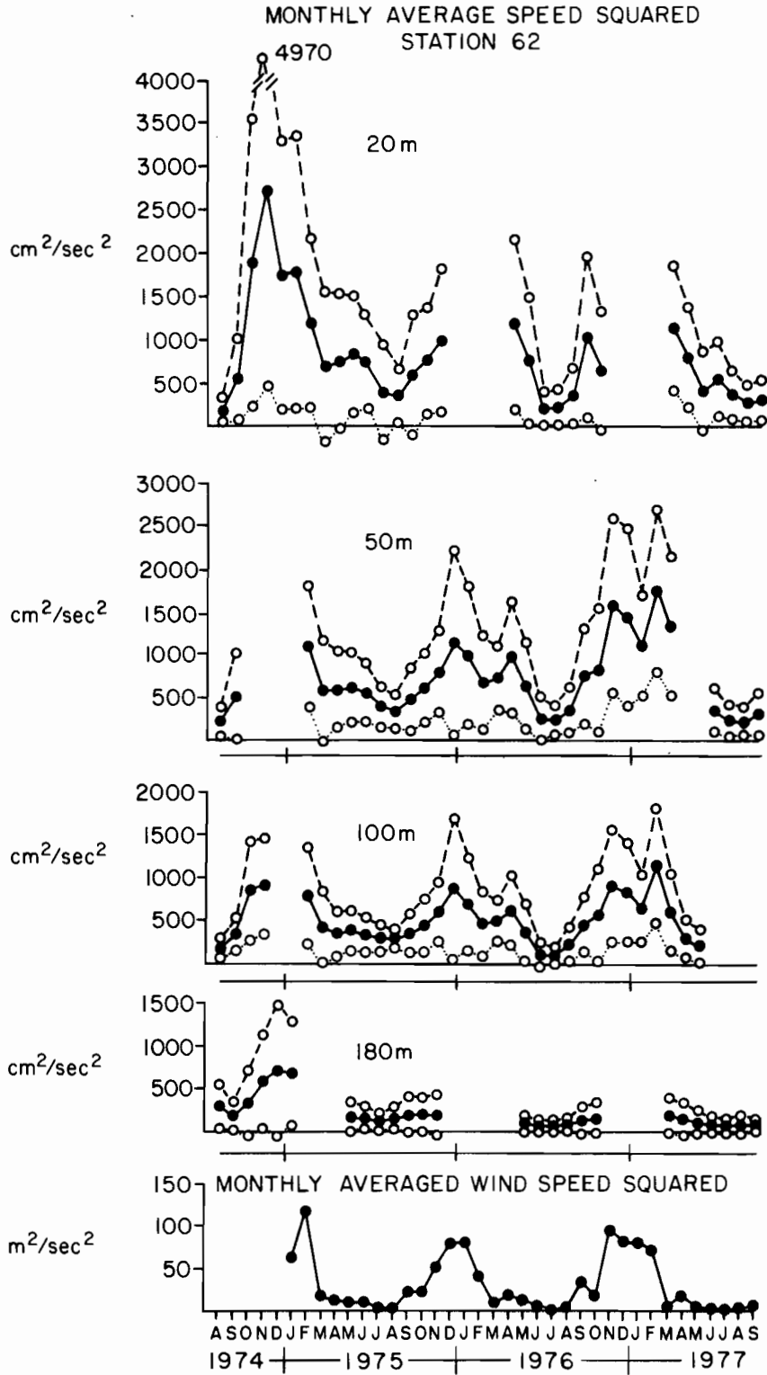
Figure 13. Average of current and geostrophic wind speeds squared, showing standard deviation as envelopes.
