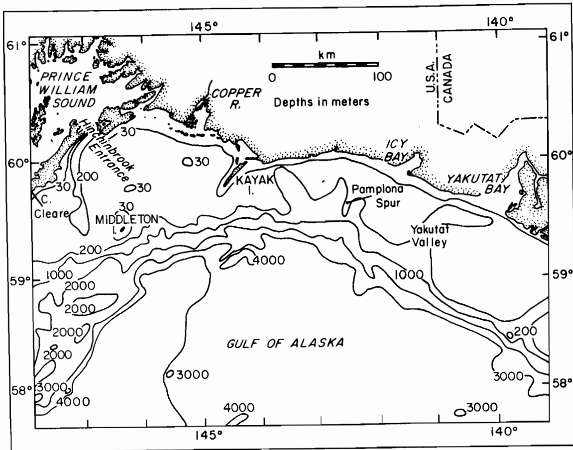
Figure 1. Geographical location in the northeast Gulf of Alaska.
