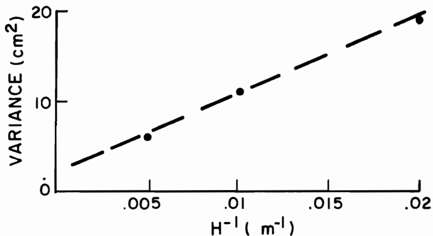
Figure 24. Low-frequency bottom pressure variance plotted as an inverse function of water depth H . A linear trend was removed from the time series before computing variance.
