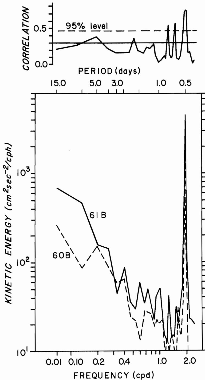
Figure 35. Kinetic energy spectra and rotary correlations for 100-m winter current records at stations 60 and 61 west of Kayak Island.
