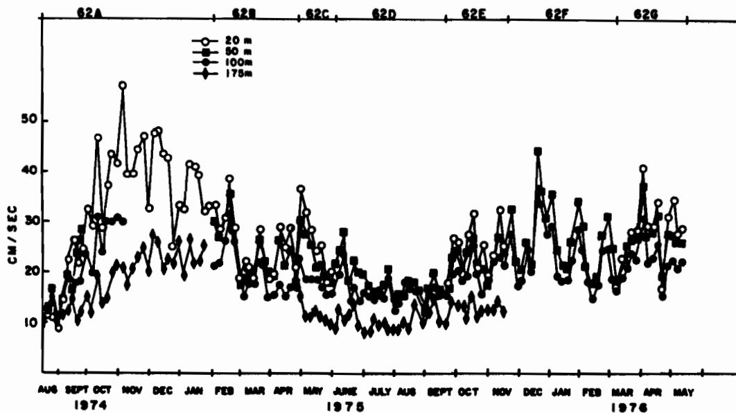
Figure 16. Five-day speeds for data from station 62 from August 1974 through May 1976. Data from the 50-m and 100-m current meters were continuous from February 1975 through May 1976. Mean speeds were higher in winter than in summer.
