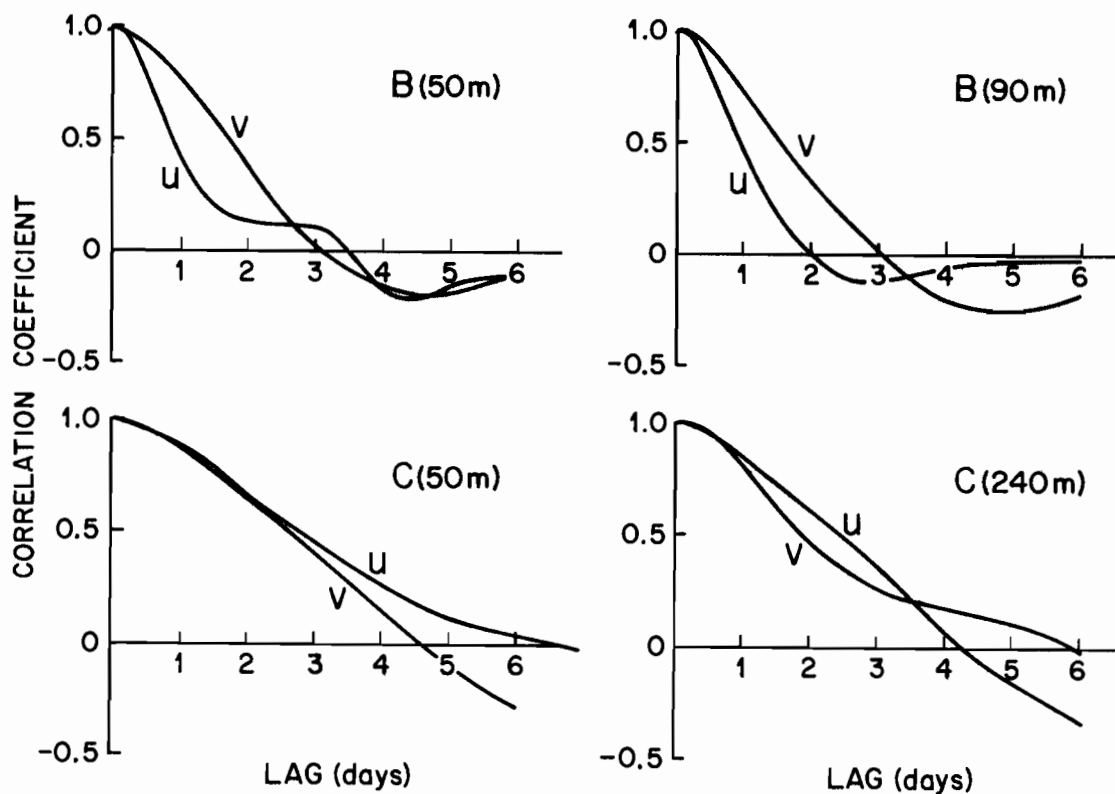
Figure 25. Autocorrelation functions of the low-pass filtered velocity components at B and C. Results for records at 50-m depth and at 10 m above the bottom are shown in each case.
