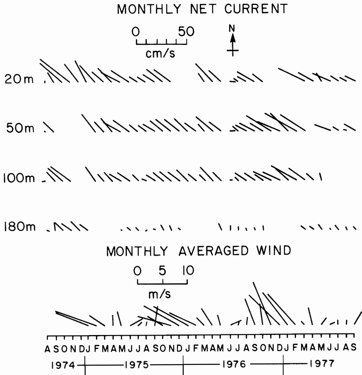
Figure 9. Monthly mean vector-averaged currents at station 62 (upper) and monthly mean averaged Bakun winds at the same location.
