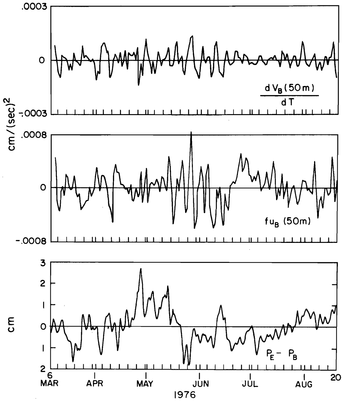
Figure 30. Acceleration of the alongshore velocity compared with the cross-shelf velocity and the alongshelf bottom pressure difference. Measurements were made at the 100-m isobath. Velocity records are from 50-m depth; f is the Coriolis parameter.
