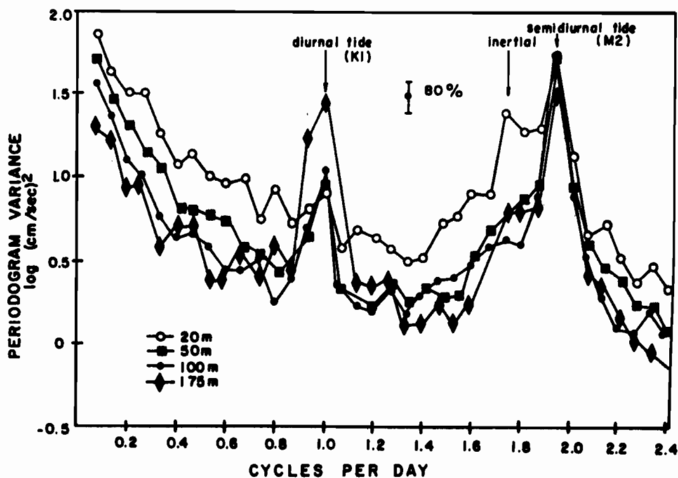
Figure 17. Ensemble-averaged energy spectra for the station 62 data. Tidal and inertial frequencies are denoted. Energy is given by logarithm of periodogram variance.
