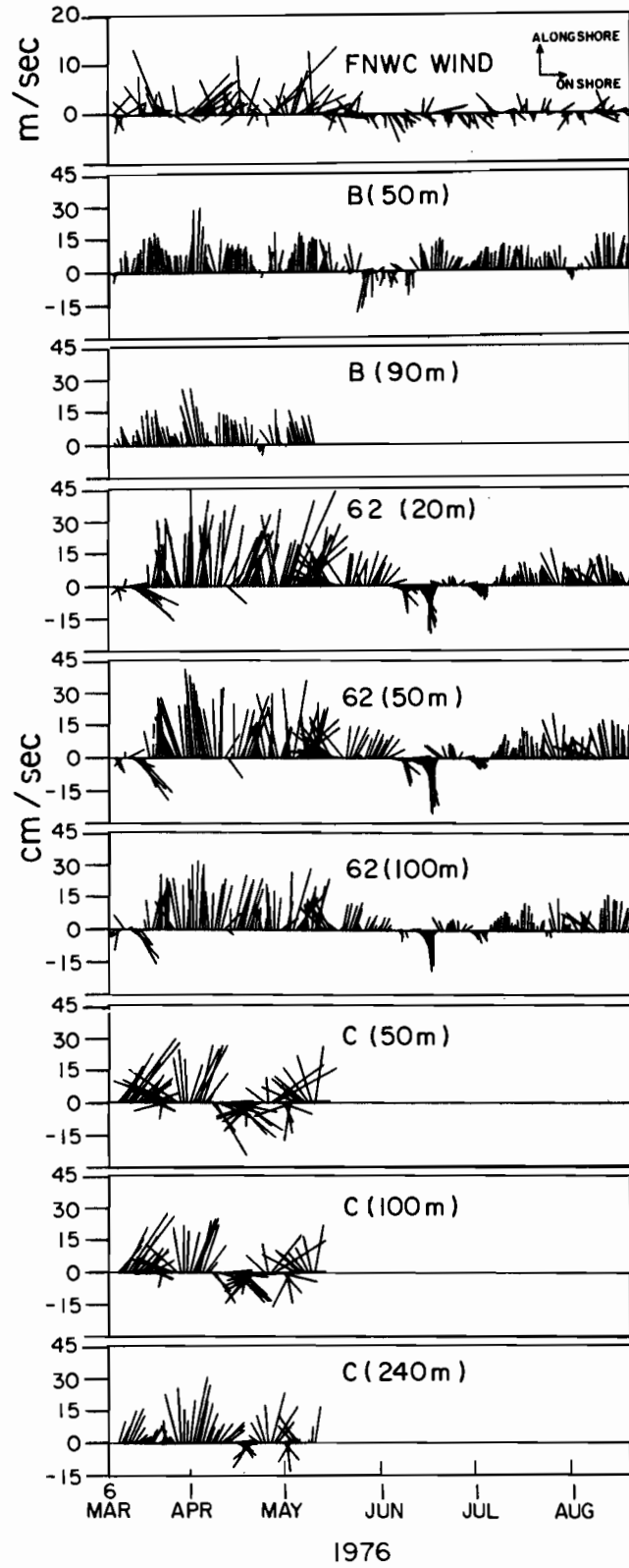
Figure 22. FNWC vector time series for the calculated wind and measured currents. All vectors have been low-pass filtered and rotated into along-shore and onshore axes as discussed in text.
