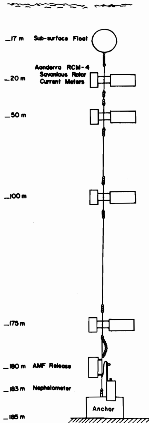
Figure 5. Schematic diagram showing configuration of current moorings used in the northeast Gulf of Alaska (from Feely et al., 1978). Where pressure gages were used, they replaced the nephelometer.
