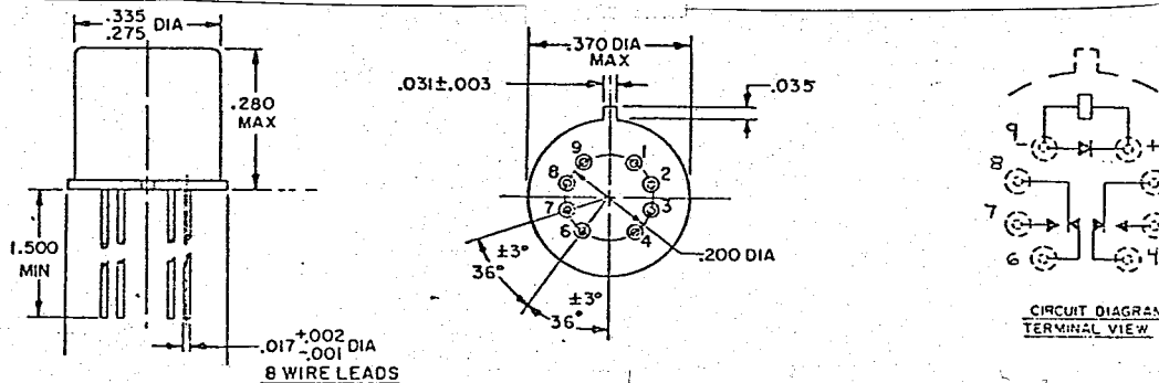
Figure 1. Configuration and circuit diagram.
