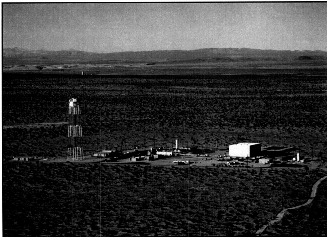
Figure 5.—X-33 Launch Facility—Haystack Butte, Edwards AFB.
