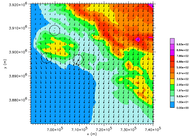
Figure 3: Diablo Canyon winds at \sigma_z = 0.208 . Every other wind vector is plotted. The circles indicate the location of the three sodar observations.
