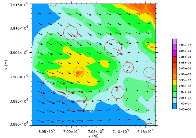
Figure 2: Enlargement of the wind field from previous figure surrounding the release site. Every other wind vector is plotted.
