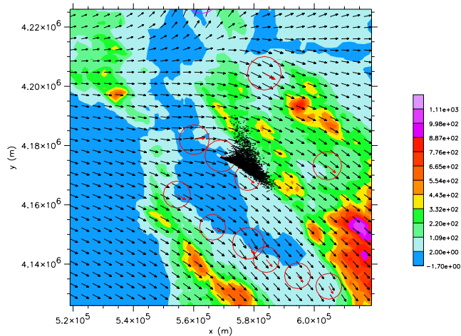
Figure 5: Surface wind field at 10 m AGL. Every third wind vector is plotted. The circles indicate the location of surface wind observations.
