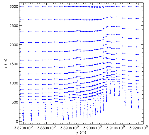
Figure 4: Diablo Canyon y - z cross section of the wind field. The vertical wind component is exaggerated by a factor of ten.
