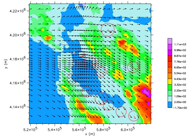
Figure 6: Surface wind field on a graded mesh at 10 m AGL for the same data as in the previous figure. Every third wind vector is plotted.
