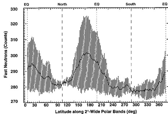
Fig. 7. Averages and standard deviations of all fast-neutron counts for all equal area pixels in figure 3 of (22) within successive 2° wide latitude bins that are banded in azimuthal angle by planes that are parallel to the lunar polar axis and separated by 2° in longitude at the equator.
