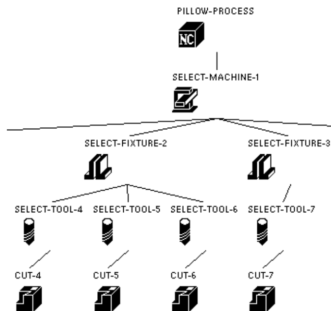
This illustration shows a portion of a process plan on NextCut.
