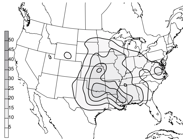
Figure 9: Same as Fig. 8, except for smallest coverage period.
