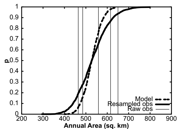
Figure 7: CDF of mean annual areal coverage, in square kilometers, of F2 or greater tornadoes based on 15-year subperiods. Dashed line from Monte Carlo simulation, thick solid line from resampled observations, and thin vertical lines from non-overlapping periods in raw observations.
