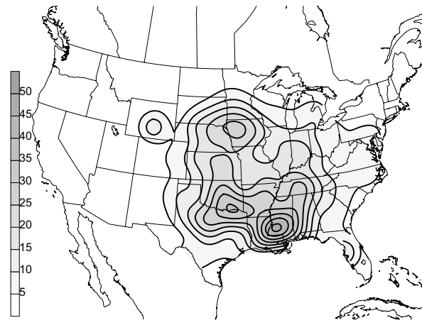
Figure 8: Percent areal coverage of grid boxes for largest coverage 15-year period from Monte Carlo simulation.
