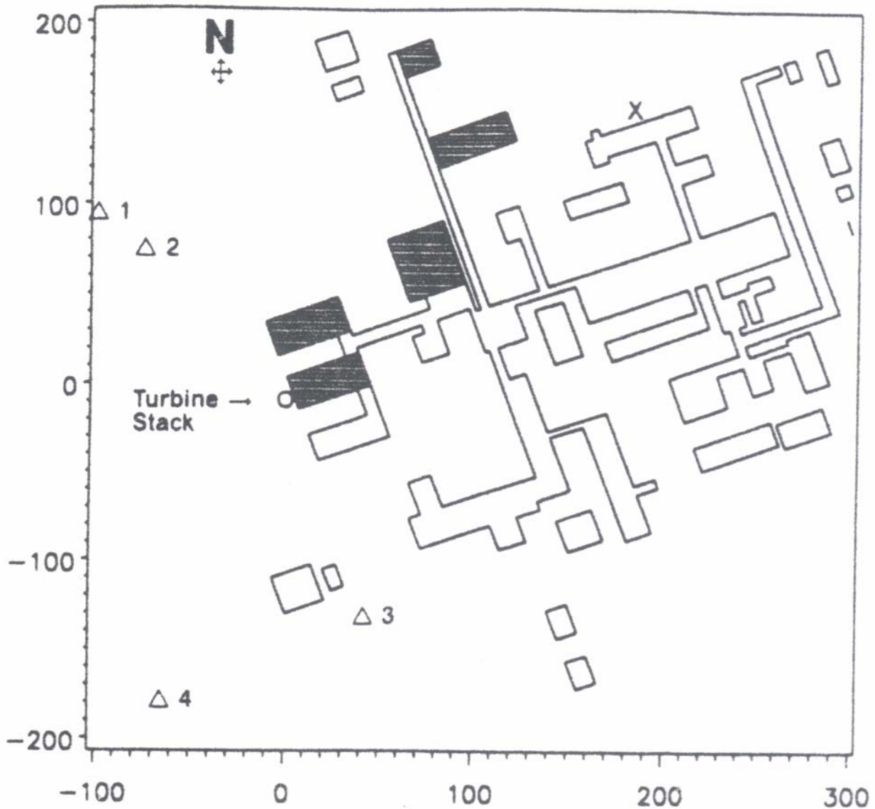
Figure 4. Depiction of Alaska North Slope Oil Gathering Center Turbine Stack, Meteorological Tower (X), and Camera Locations Used to Visualize Plume Rise 43
