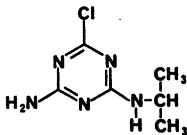
2-Amino-4-chloro-6-isopropylamino-s-triazine
