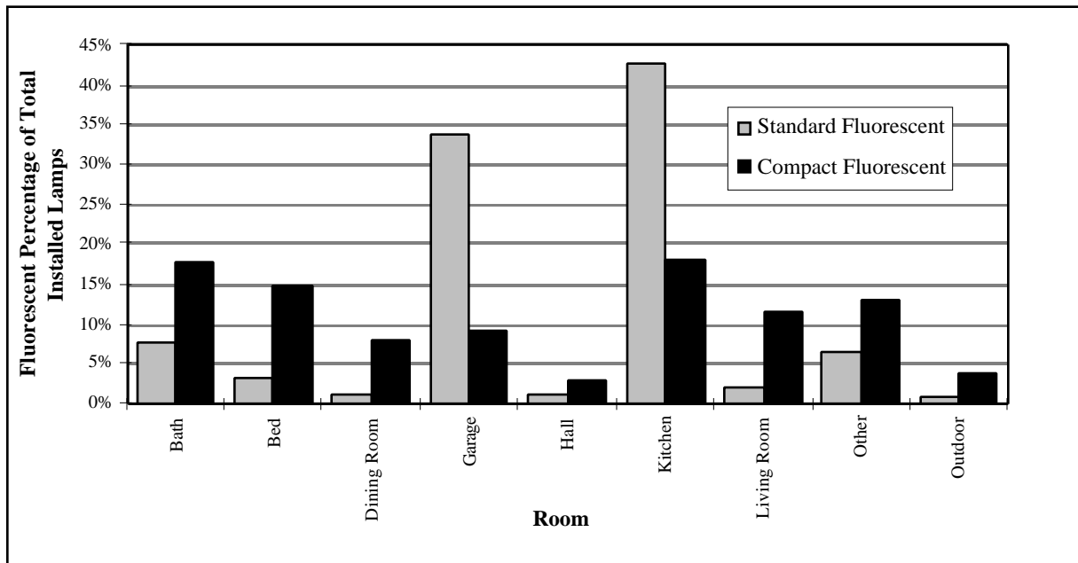
Figure 1.8: Fluorescent Lamp Saturation—PG&E Service Territory
