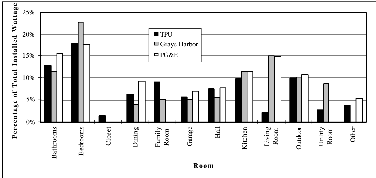
Figure 1.2: Percentage of Installed Wattage, by Room Type
