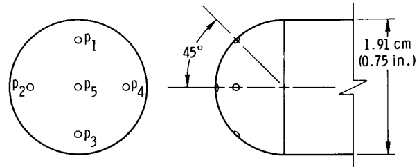
Figure 2. Location of ports in probe tip.
