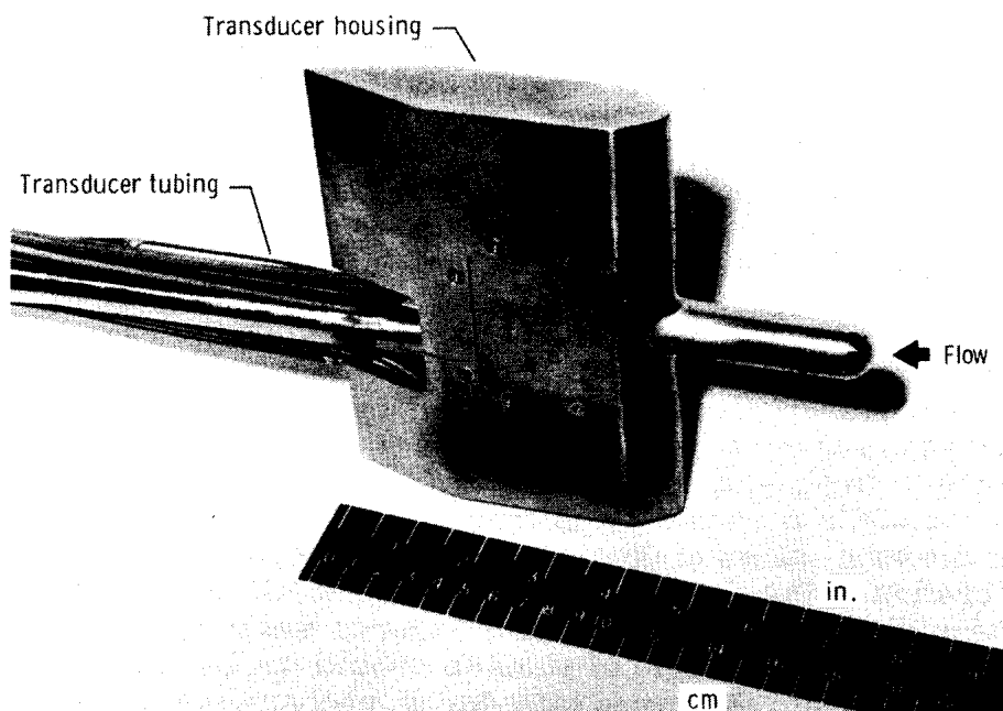
Figure 1. Hemispherical head flow direction sensor.
