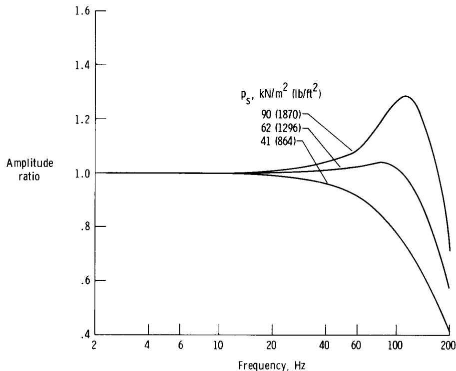
Figure 3. Frequency response of hemispherical head flow direction sensor.
