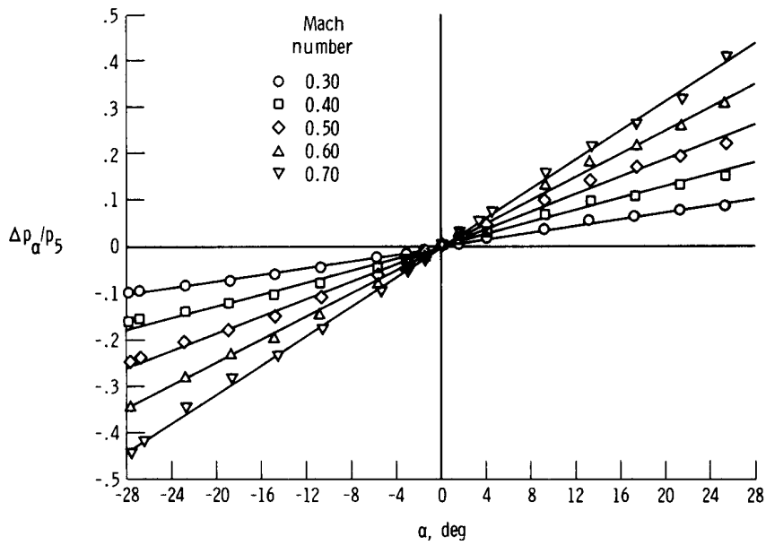
Figure 9. Variation of \Delta p_\alpha/p_5 with angle of attack and Mach number. \beta \approx 0^\circ ; \varphi \approx 0^\circ ; R = 4.92 \times 10^6 per meter ( 1.5 \times 10^6 per foot).
