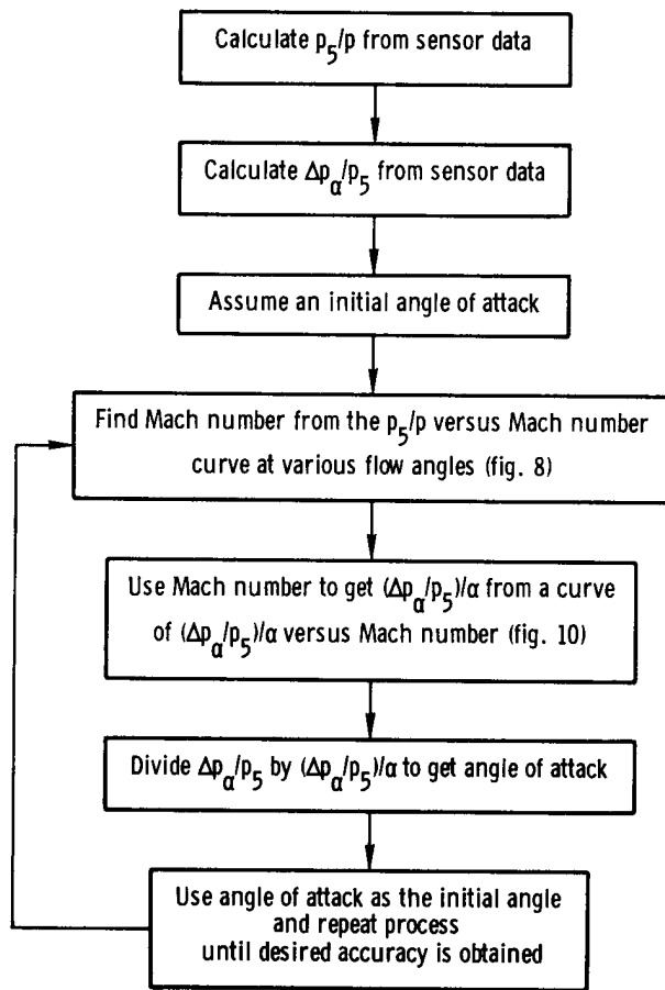
Figure 11. Procedure for calculating angle of attack and Mach number by using method 3.
