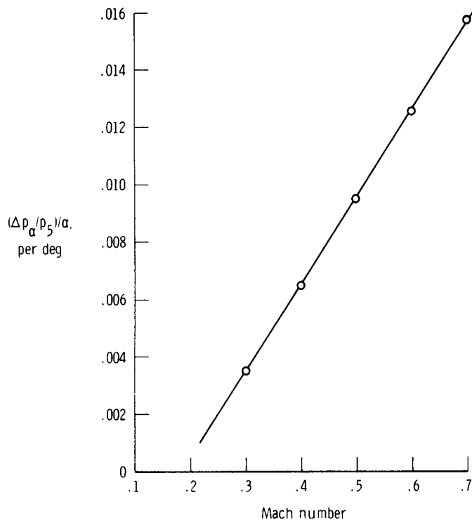
Figure 10. Variation of (\Delta p_\alpha/p_5)/\alpha with Mach number. \beta \approx 0^\circ ; \varphi \approx 0^\circ ; R = 4.92 \times 10^6 per meter ( 1.5 \times 10^6 per foot).
