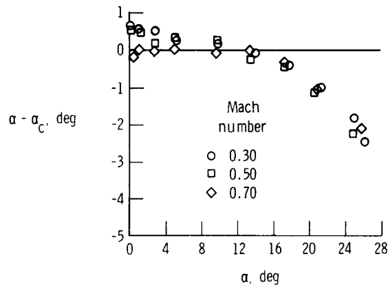
Figure 6. Angle of attack correction curve for a roll angle of 21.5^\circ . \beta \approx 0^\circ ; R = 4.92 \times 10^6 per meter ( 1.5 \times 10^6 per foot).
