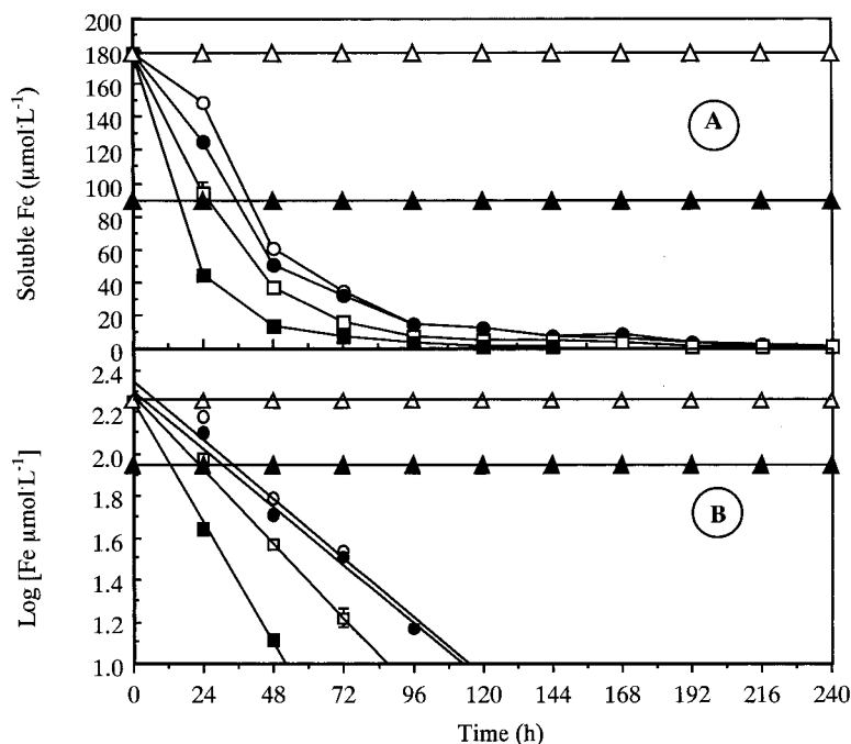
Fig. 4. (A) Loss of soluble Fe in linear plot vs. time and (B) linear regression profile of the logarithm of soluble Fe ( \mu\text{mol}\cdot\text{L}^{-1} ) vs. time (h) for 5× or 10× lab-prepared nutrient solutions containing FeDTPA or FeEDTA ( 14.28 \text{ mmol}\cdot\text{L}^{-1} \text{ N} , 17.9 \text{ }\mu\text{mol}\cdot\text{L}^{-1} \text{ Fe} = 1×). Nutrient solutions (20 °C or 40 °C) were irradiated with a fluorescent plus incandescent light source providing 250 \text{ }\mu\text{mol}\cdot\text{m}^{-2}\cdot\text{s}^{-1} or 500 \text{ }\mu\text{mol}\cdot\text{m}^{-2}\cdot\text{s}^{-1} (330–800 nm) measured at the outer surface of the container. Treatments were: 1) FeEDTA, 10×, 20 °C, 250 \text{ }\mu\text{mol}\cdot\text{m}^{-2}\cdot\text{s}^{-1} (●); 2) FeDTPA, 10×, 20 °C, 250 \text{ }\mu\text{mol}\cdot\text{m}^{-2}\cdot\text{s}^{-1} (○); 3) same as 2) but wrapped in aluminum foil (△); 4) same as 2), but at 40 °C (□); 5) same as 2), but at 500 \text{ }\mu\text{mol}\cdot\text{m}^{-2}\cdot\text{s}^{-1} (■); 6) same as 5), but 5× and under spectral filter Acrylic yellow-2208 (▲). All containers were 1 L except for the 5× treatment, which was a 500-mL container. Vertical bars indicate SE ( n = 3 ). If none are shown, they fall within the dimensions of the plotting symbol.
