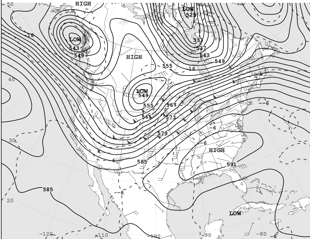
SUN, JUN 08, 2008 500-Millibar Height Contours at 7:00 A.M. E.S.T.
