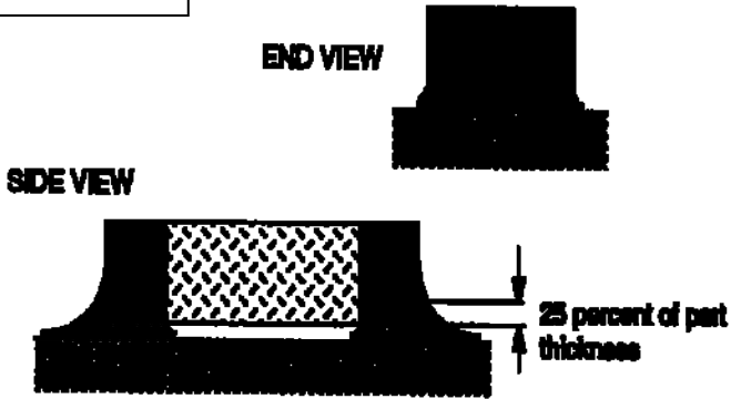
Figure B-2: Chip Part Tilting
