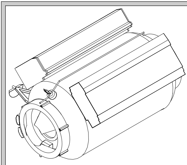
Figure 9a. The Russian-designed Docking Module which was added to Kristall in November 1995 to accommodate future Space Shuttle dockings with the Mir complex. An APAS mechanism shows at the end of the module (left side of drawing). The module was transported to Mir by Atlantis on STS-74.
