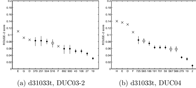
Fig. 5. ROUGE-2 recall scores plotted with 95% confidence intervals (lines) for the human ( \times ), summarization module ( \circ ), and QCS ( \bullet ) summaries for the d31033t clusters in the DUC03-2 and DUC04 collections. The scores appear in descending order of average score from left to right.
