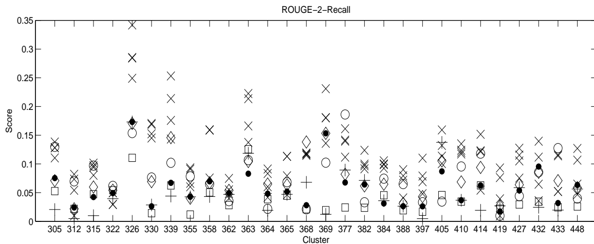
Fig. 7. ROUGE-2 recall scores for DUC03 Task 4 data for the human (×) and summarization module (○) summaries, along with the top scoring QCS (●), QL (□), QS (+), and CS (◇) summaries.
