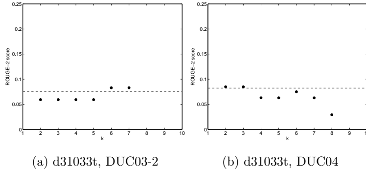
Fig. 6. Best ROUGE-2 recall scores for the QCS summaries for the d31033t clusters in the DUC03-2 and DUC04 collections as a function of the number of clusters formed ( k ). The dotted lines represent the best corresponding scores for the summarization module summaries.
