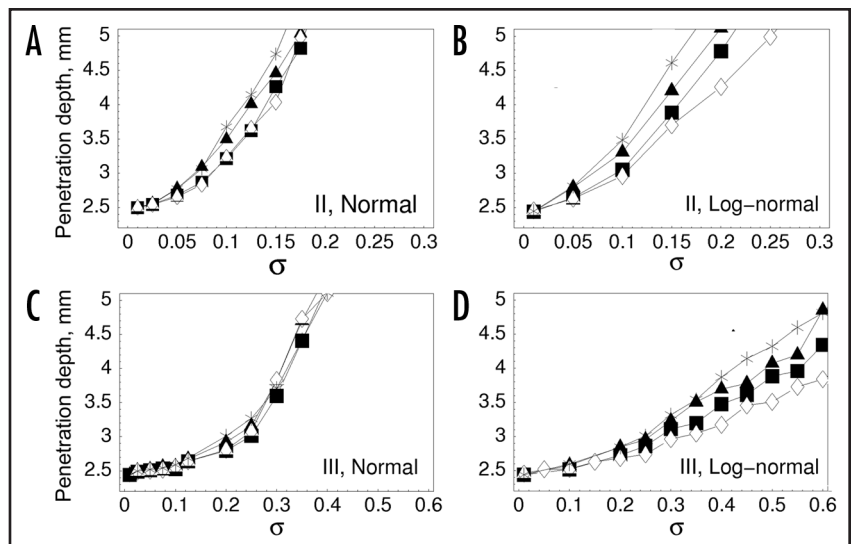
Figure 5. Modest variability in 3' PI phosphatase expression enhances wound invasion rate. In each plot, either 3' PI phosphatase expression p_{\text{max}} was varied alone (open diamonds) or together with r_{\text{max}} (filled squares), e_{\text{max}} (filled triangles), or both r_{\text{max}} and e_{\text{max}} (stars) according to sampling models illustrated in Figure 3B. Penetration depth is defined as in Figure 3. Values are averaged over 50 independent model runs, and 95% confidence intervals are within 5% of the mean, except where the penetration depth approaches 5 mm. (A) model II, normal distribution. (B) model II, lognormal distribution. (C) model III, normal distribution. (D) model III, lognormal distribution.
