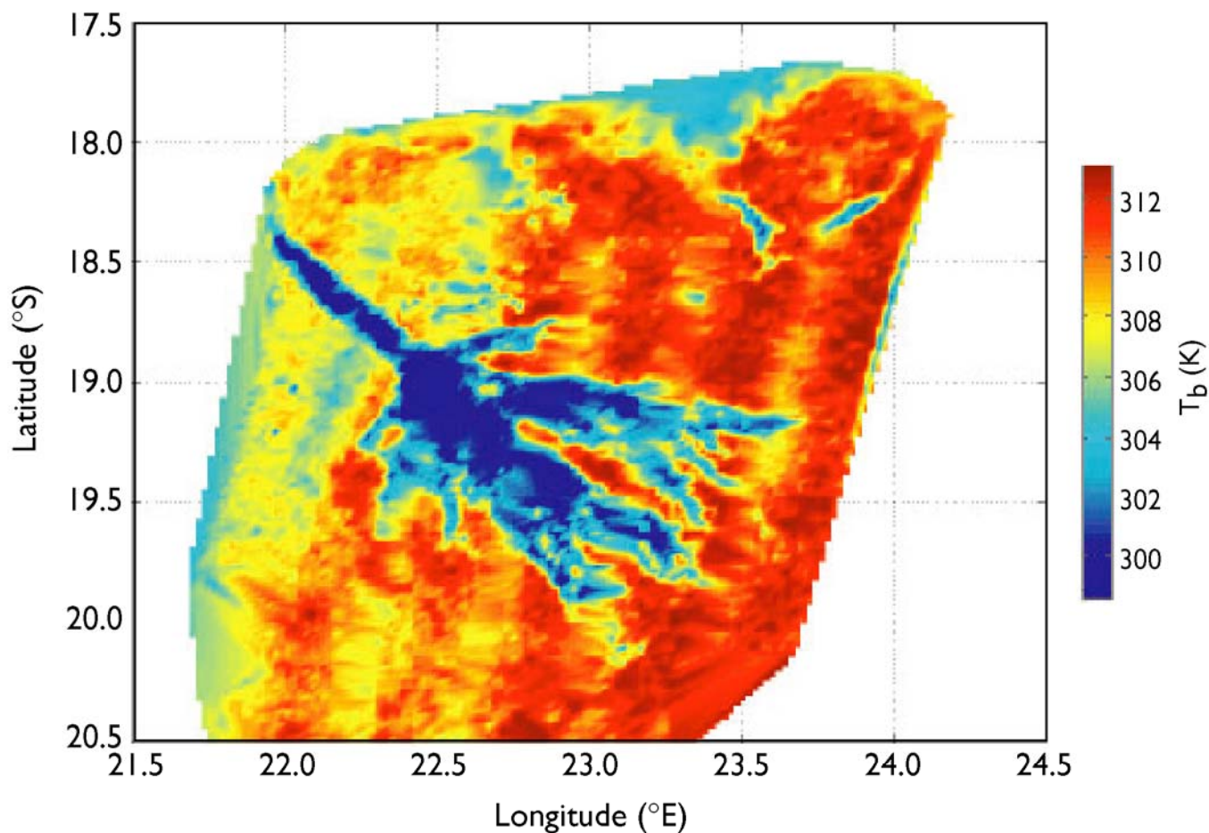
Plate 5. Brightness temperature of the Okavango Delta, Botswana at 10.2 \mu\text{m} , acquired by Scanning HIS during 6 parallel flight lines over the Delta on August 27, 2000. The pixel resolution of S-HIS is 2 km at nadir.
