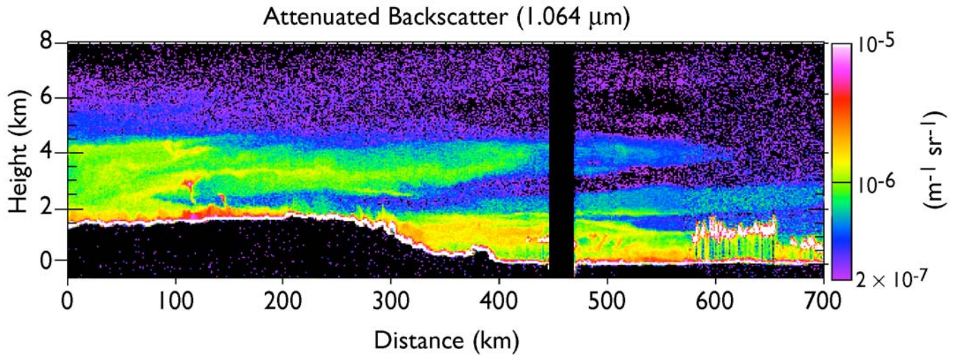
Plate 7. CPL observations of attenuated backscatter coefficient at 1.064 \mu\text{m} on August 24, 2000 obtained as the ER-2 aircraft flew from the highveld west of Witbank, South Africa, over the escarpment to Inhaca Island, Mozambique and then turned north over nearby Maputo Bay parallel-ing the Terra ground track. The multiple layers of smoke and haze are clearly evident in this plate.
