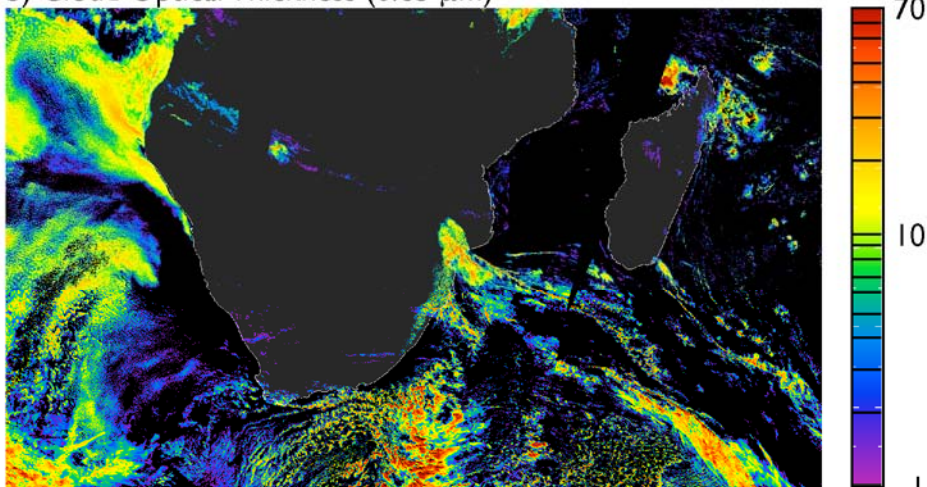
c) Aerosol Optical Thickness (0.56 μm)
