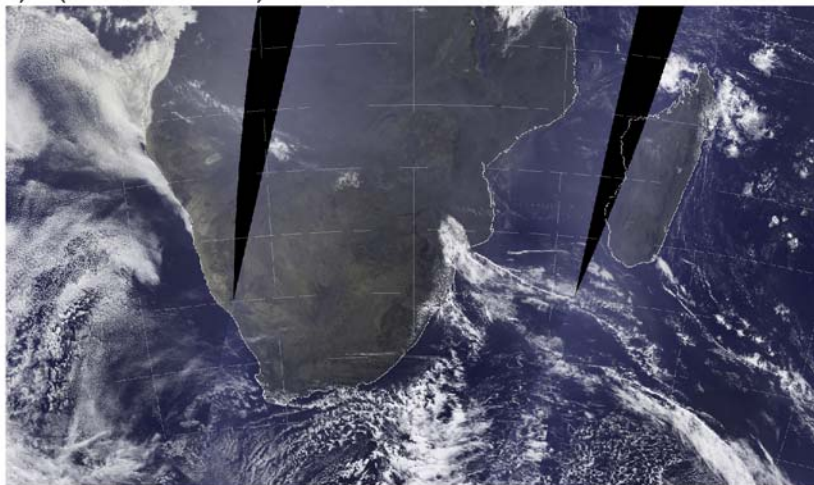
b) Cloud Optical Thickness (0.65 μm)
