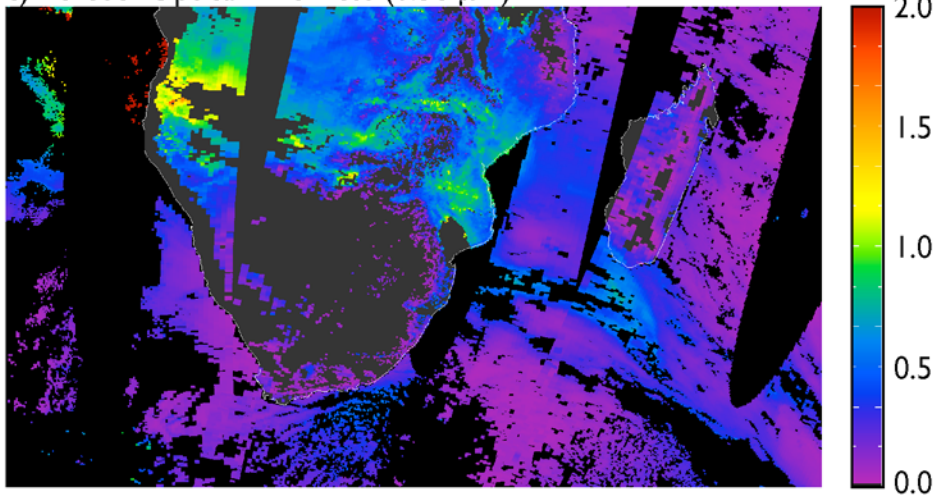
c) Aerosol Optical Thickness (0.56 μm)
