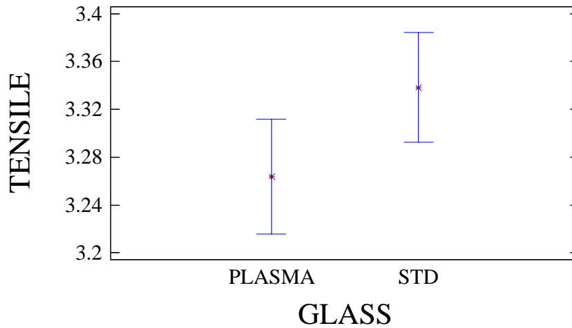
Figure 6. Tensile Strength Testing Showed No Statistically Significant Differences Between Plasma-Melted Glass And Standard Glass
