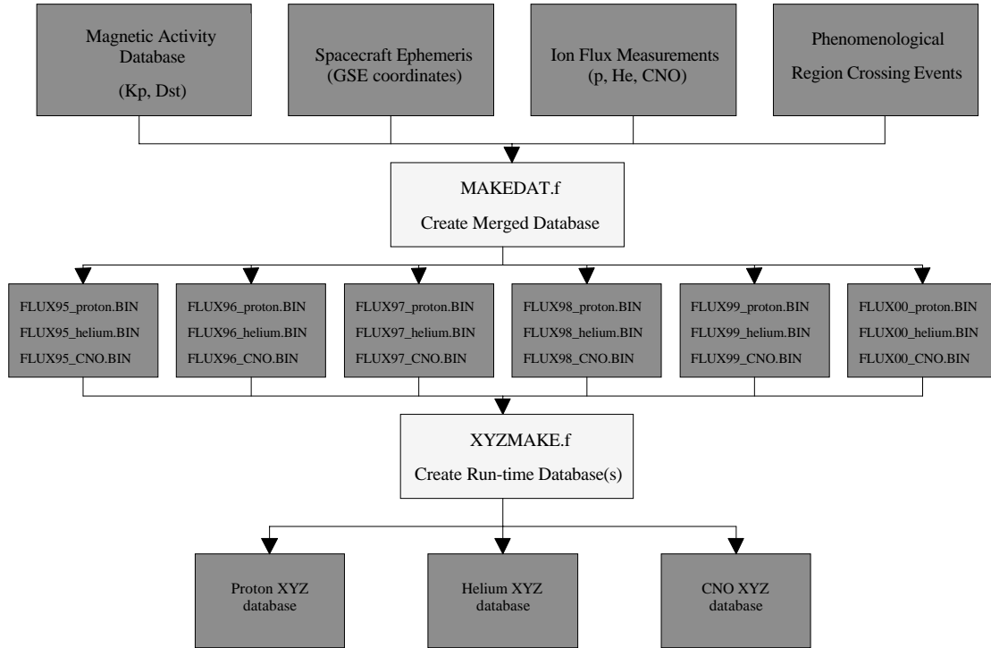
Figure 4. Schematic of Process Required to Create the Ion Flux Database. Time tagged ion flux measurements and ephemeris records from the EPIC/ICS instrument along with geomagnetic indices (Kp, Dst) and identification of the plasma regimes (solar wind, magnetosheath, or magnetosphere) are combined to create a merged database for individual years. This database is then processed into individual runtime databases of ion flux (proton, helium, or CNO).
