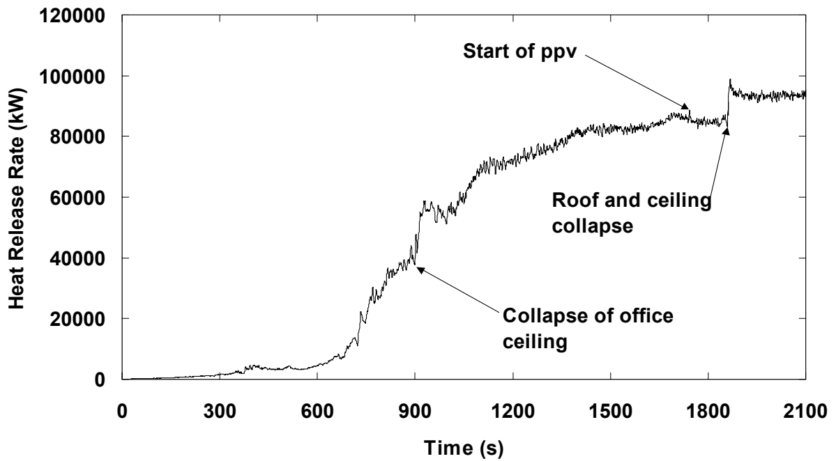
Figure 20. Heat release rate for simulation.
