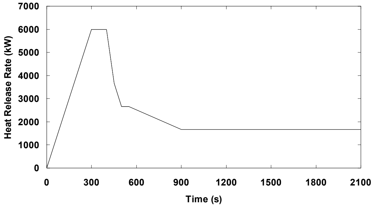
Figure 7. Heat release rate for the ignition source.
