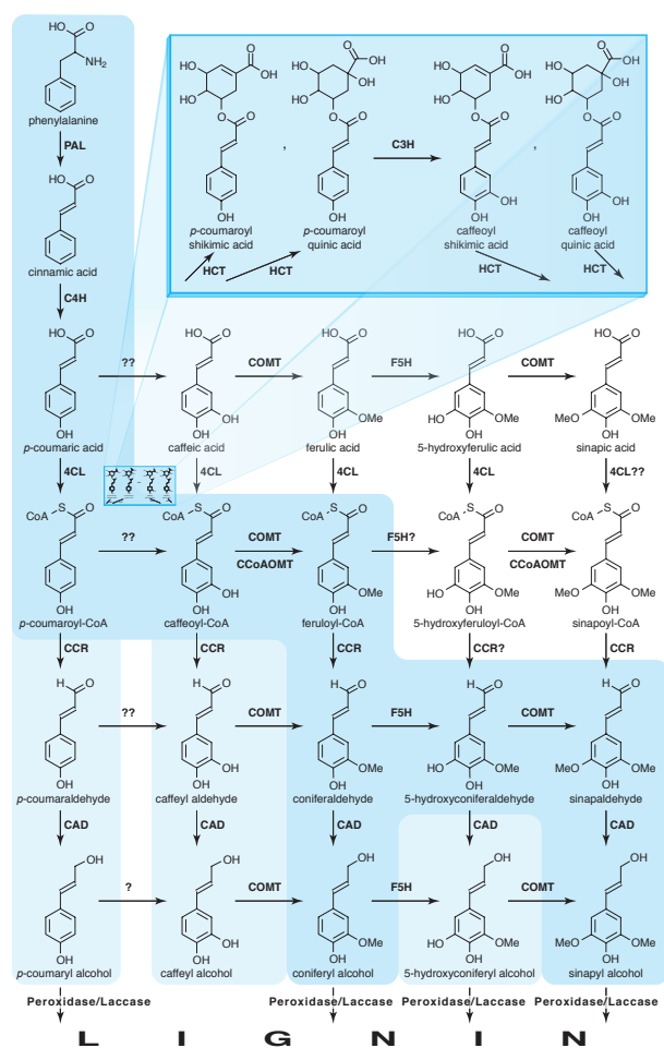
Fig. 1. Simplified monolignol biosynthetic pathway. 1 Note that, at least in Arabidopsis, the p -coumaric acid to caffeic acid conversion involves more steps than previously thought, as shown in the expansion. Traditional names for the enzymes involved are: 4CL = 4-coumarate:CoA ligase; C3H = p -coumarate 3-hydroxylase; HCT = p -hydroxycinnamoyl-CoA: quinate shikimate p -hydroxycinnamoyltransferase; CCoAOMT = caffeoyl-CoA O -methyltransferase; CCR = cinnamoyl-CoA reductase; F5H = ferulate 5-hydroxylase; CALd5H = coniferaldehyde 5-hydroxylase; COMT = caffeic acid O -methyltransferase; AldOMT = 5-hydroxyconiferaldehyde O -methyltransferase; CAD = cinnamyl alcohol dehydrogenase. Many of these enzymes are no longer thought to function on the substrates for which they were originally named.
