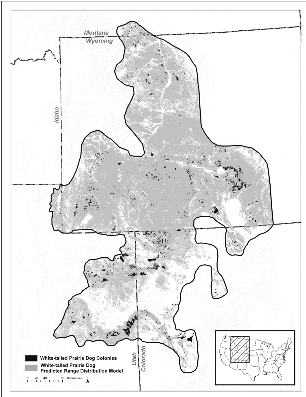
Figure 1: North American range and potential distribution of white-tailed prairie dogs reproduced from Seglund et al (2004). Solid black lines delineate the probable extent of prairie dog range. Gray areas represent the subset of this range that is deemed possible of containing prairie dogs based on a simple overlay of habitat type, elevation, slope, and major disturbances. Black areas represent rough outer limits of historic and current prairie dog colonies identified by state wildlife agencies.
