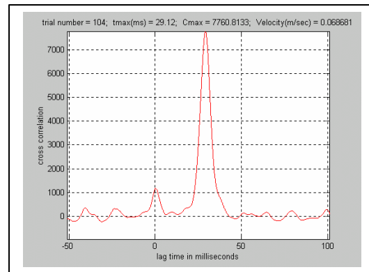
Figure 3b: Cross Correlation of S_1(t) and S_2(t) . Delay, t_d = 29\text{ms} . Given d = 2\text{mm} , V_x = 6.9\text{ cm/s} .
