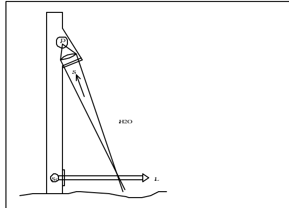
Figure 1b: Detector Configuration.
