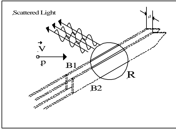
Figure 1a: Particle Crossing Ribbon Pair.
