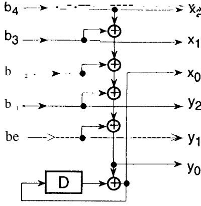
Fig. 10. Optimum 2-state inner trellis encoder for SCTCM with 2x 8PSK Modulation,
