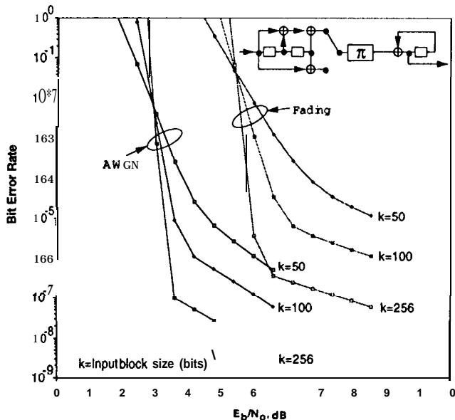
Fig. 8. Performance of rate 1/2 SCCC over AWGN and Rayleigh Fading Channel
