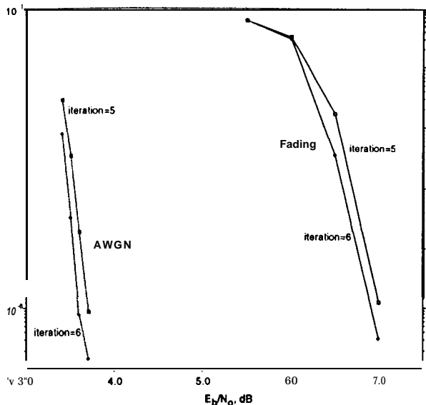
Fig. 6. BER Performance of Parallel Concatenated Trellis Coded 8PSK, 2 bits/sec/Hz,
