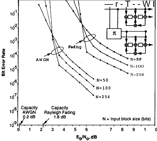
Fig. 3. Performance of rate 1/2 PCCC over AWGN and Rayleigh Fading Channel
