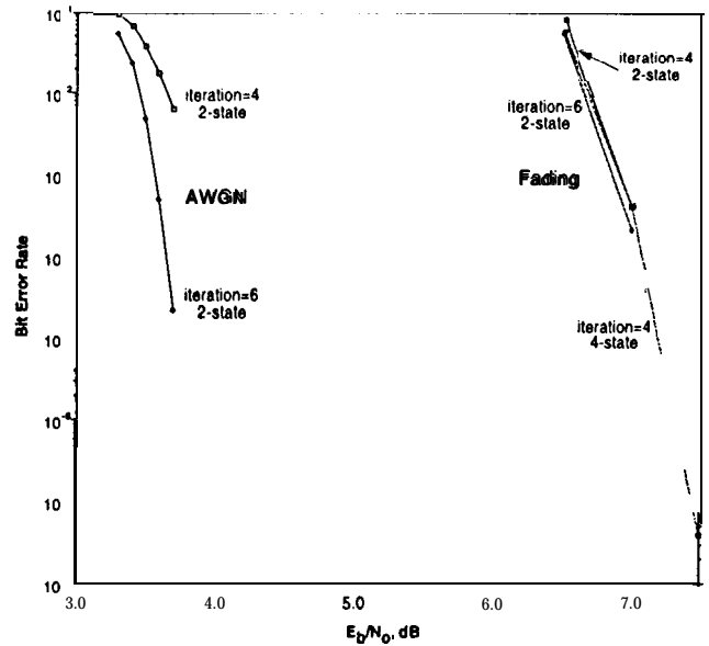
Fig. 12. Performance of Serial Concatenated Trellis Coded Modulation, 8-state outer 2-state or 4-state inner with 2x8PSK, 2 bits/see/Hz
