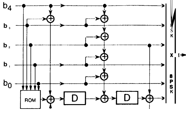
Fig. 11. 4-state inner trellis encoder for SCTCM with 2x8PSK modulation for Rayleigh fading.
