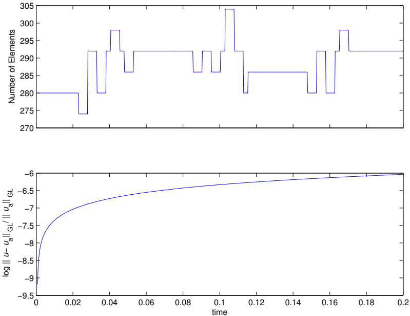
Fig. 9. Plots of diagnostic quantities vs time in the p = 8 linear advection test. Top : number of elements vs time. Bottom : \log_{10}(\|\mathbf{u} - \mathbf{u}_a\|_p / \|\mathbf{u}_a^0\|_p) vs time . The errors for the adaptive and control meshes lie on top of one another.
