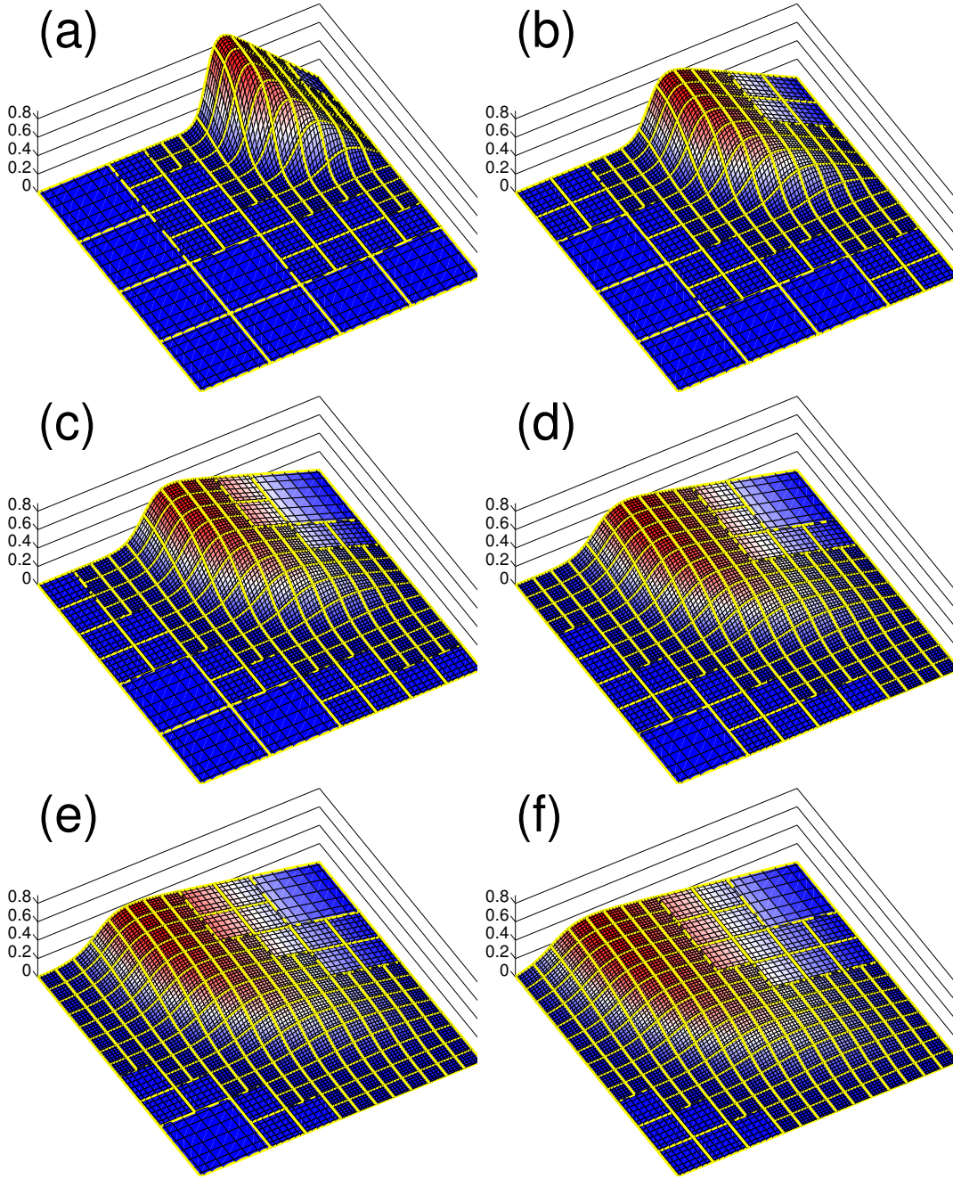
Fig. 10. Surface plots of u^1(\vec{x}, t) solved from (1), showing \vec{x} \in [\frac{1}{2}, 1]^2 and K/4 = 88 , 121, 139, 172, 181, 190 as t = 0.18, 0.33, 0.48, 0.65, 0.81, 1.00 . Here \vec{c} = \vec{u} , \nu = 5 \times 10^{-3} , p = 8 , and (21) is the initial condition.
