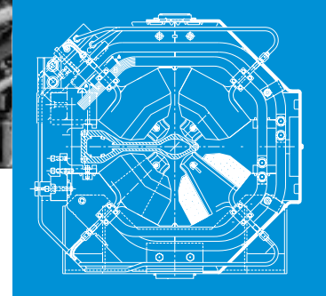
↑ A computer-aided drawing of an APS storage ring quadrupole magnet face. Three lengths of quadrupole magnets are used at different locations in the storage ring; 80 are 0.8 m, another 80 are 0.6 m, and 240 are 0.5 m. They focus (control the size of) the positron beam, much like a lens focuses light.
