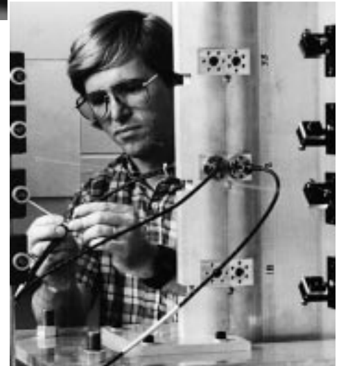
↓ Storage ring beam position monitor buttons mounted on a section of aluminum-alloy storage ring vacuum chamber for testing.
