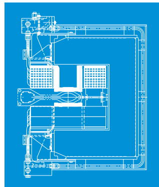
← The face of an APS storage ring dipole magnet. Dipole magnets steer the particle beam on a closed orbital path. Half of the 80 storage ring dipoles can provide radiation to experimenters via beamlines.
