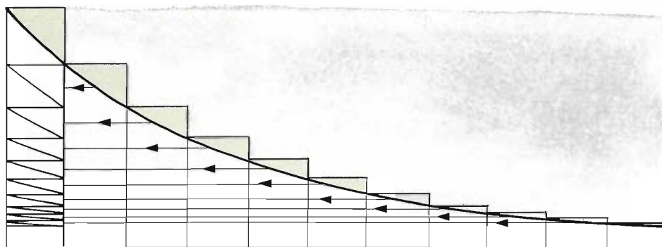
Fig. 1. K. Kuratowski posed the following problem to his calculus class: Over a non-negative, decreasing function on the positive part of the real line, construct a step function with steps of equal depth. Prove that the area of the shaded regions between the two functions is finite. Ulam's solution was to move each shaded region into the first column, the area of which is finite.
