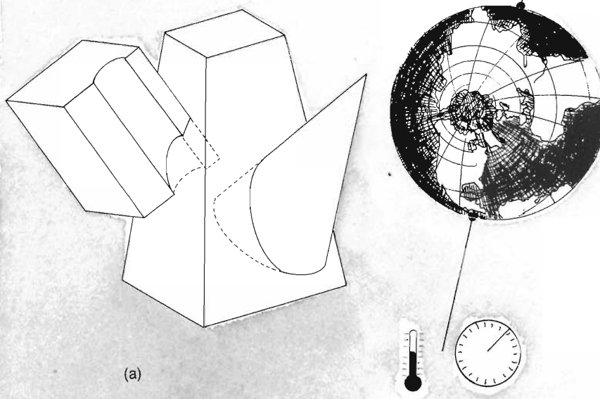
Fig. 3. You can divide the volumes of any three bodies in half with a single plane (not shown) even when the bodies intersect. (b) You can always find antipodes on the earth with the same pressure and temperature.
