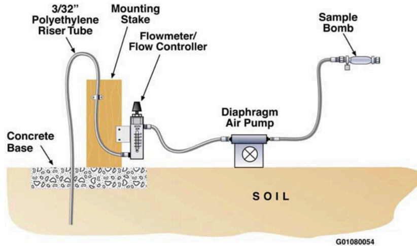
Figure 5.2. Schematic Diagram of Soil-Gas Sampling System Used for Collection of Stable Isotope Samples
