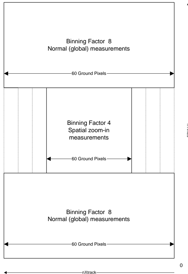
Figure 3-2 Example of Spatial Coverage for Zoom Measurements 1
