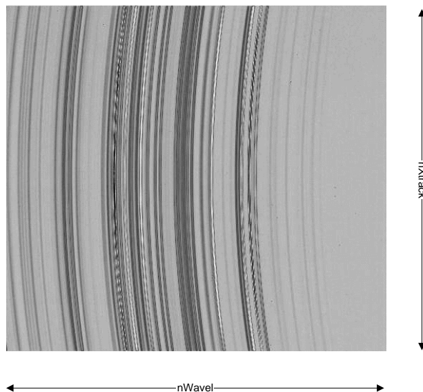
Figure 3-4 SLS measurement showing the spectral smile of OMI in the UV-2 Sub Channel
