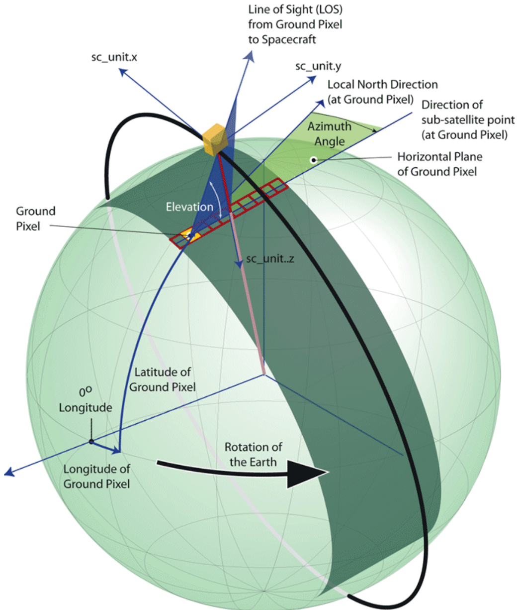
Figure 5 - Geolocation for ground pixels
