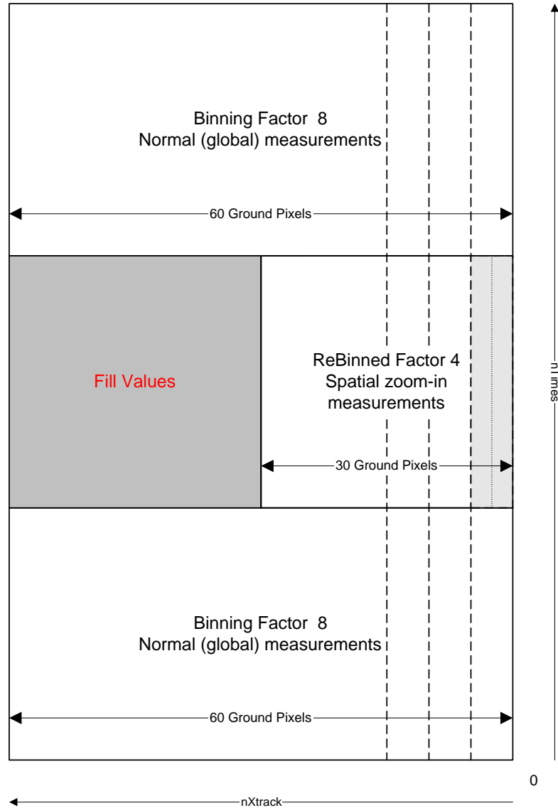
Figure 3-3 Example of Rebinned Zoom Measurements 2
