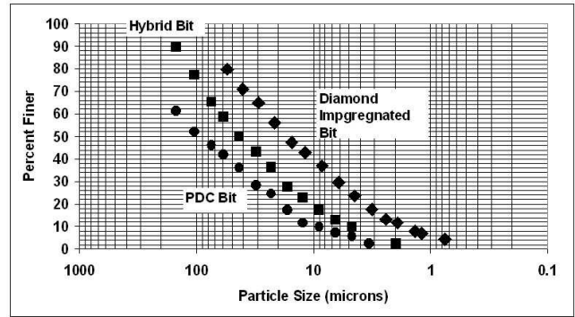
Figure 5. Particle size distribution of cuttings produced with PDC, Hybrid and Diamond Impregnated bits.
