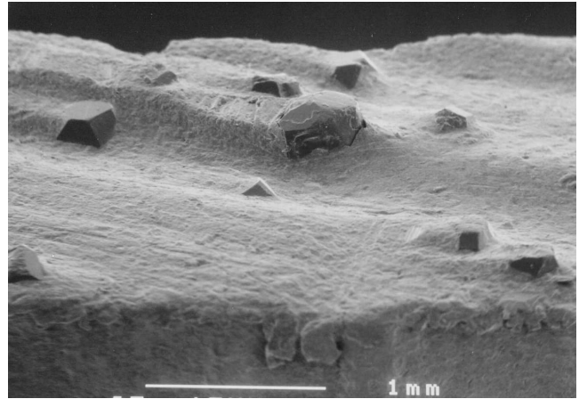
Figure 2. Scanning Electron Micrograph of a diamond impregnated segment in good condition.
