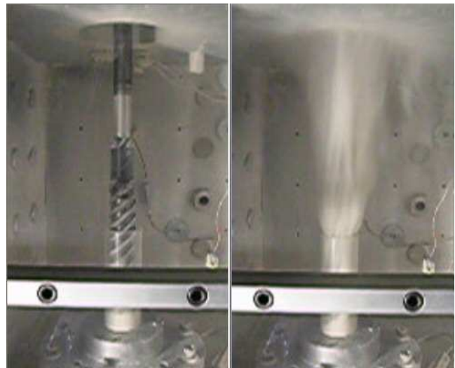
Figure 6. A view of the drill and a hole (clear acrylic tube) before and during a gas flushing.
