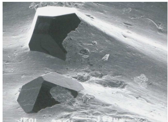
Figure 10. Diamonds are replaced before they wear when drilling in water saturated rock at 5 torr.
