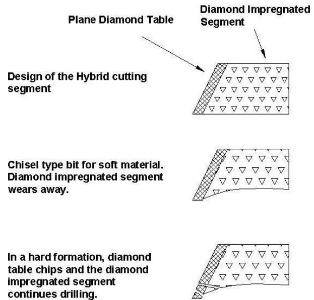
Figure 4. A hybrid, self-sharpening cutting segment for drilling in any geological formation.
