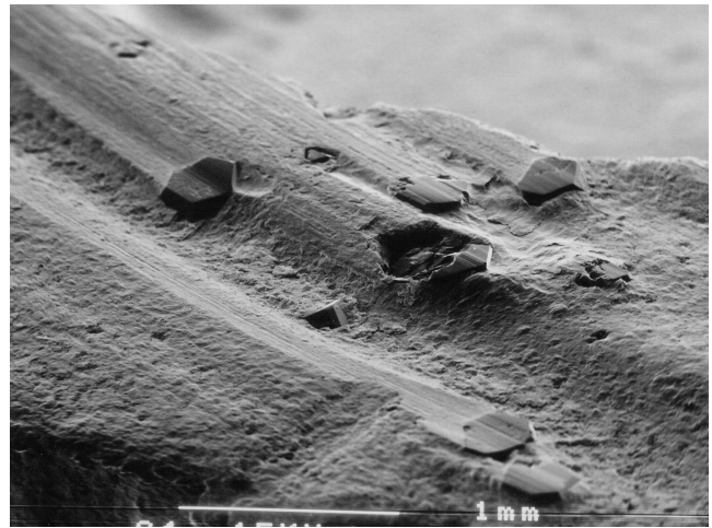
Figure 3. Scanning Electron Micrograph of an ineffective diamond impregnated segment (note polished and flattened diamonds).
