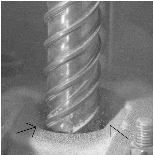
Figure 8. A close up of the drill and the hole showing rock cuttings being blown out of the hole. The auger diameter is 39 mm. ( Zacny et al. [2004])
