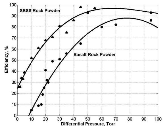
Figure 7. Extraction efficiency of the Santa Barbara Sandstone and Basalt rock powders as a function of differential pressure (after Zacny et al. [2005]).
