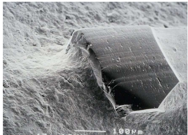
Figure 9. Diamond wear under Earth atmospheric conditions is extensive.
