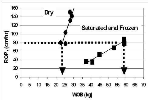
Figure 12. Rate of Penetration vs Weight on Bit for a dry and water saturated frozen sandstone under Martian pressure.
