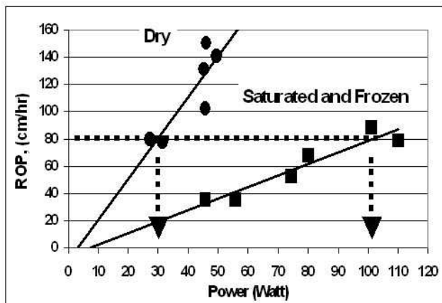
Figure 11. Rate of Penetration vs Power for a dry and water saturated frozen sandstone under Martian pressure.
