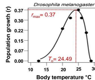
Fig 1. Example of a thermal fitness curve we obtained from the literature.
