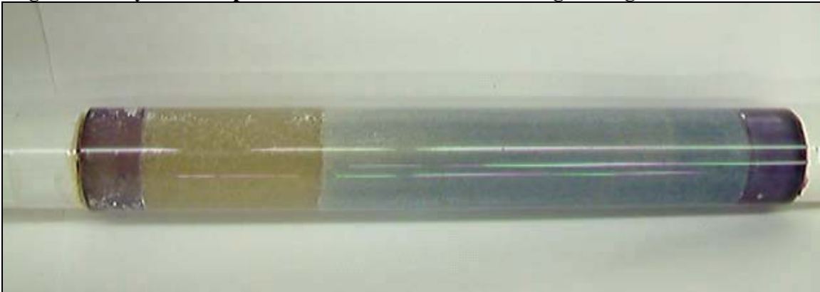
Figure 11. Dyed Transparent APHRON ICS Mud Flowing through 20/40 Sand Pack
