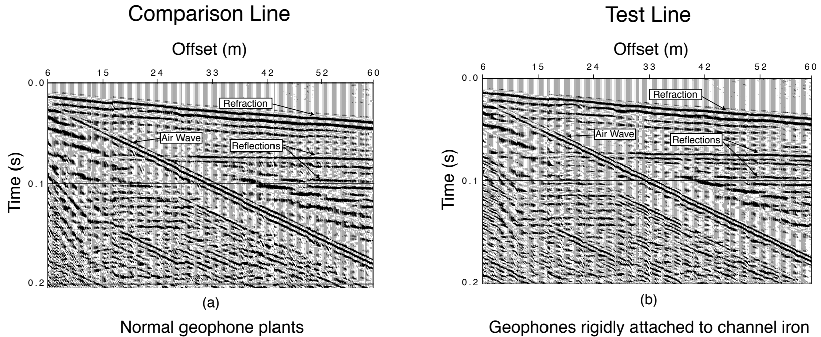
Figure 1. Comparison of walkaway wave-test data recorded using (a) geophones planted normally, and (b) geophones bolted to four, 2.7-m-long pieces of channel iron and then inserted into the ground. Note the similarities in phase and amplitude of the refractions on both records. Note also the similarity of the reflections at 72 ms and 94 ms, respectively. Also note that the 74-ms reflection can be followed continuously from ~ 15 m (inside the air wave) to 60 m for both (a) and (b), with no interfering modes visible in (b), in which the data come from geophones attached to the channel iron. The data were processed using a bandpass filter with 300-500 Hz, rolling off at 12 dB/octave and plotted with an AGC window of 25 ms. A 30.06 rifle fired into a shallow, prepunched hole provided the seismic energy recorded on both lines.
