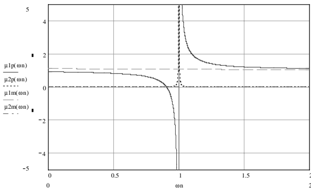
Figure 3. Complex permeability of a YIG material, 4\pi M_s = 250 Gauss, \Delta H_k = 4 Oe, \omega_n = \omega/\omega_0 .
