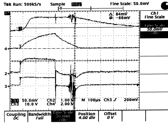
Figure 7. Measured phase shifter response. 1=phase detector output, 2=pulse transformer input voltage (x1000 probe), 3=pulse transformer output voltage, 4=phase shifter bias current (1 V for 100 A).
