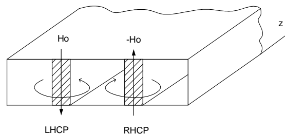
Figure 1: Two circularly polarized magnetic fields of a TE_{01} mode in a rectangular waveguide.
