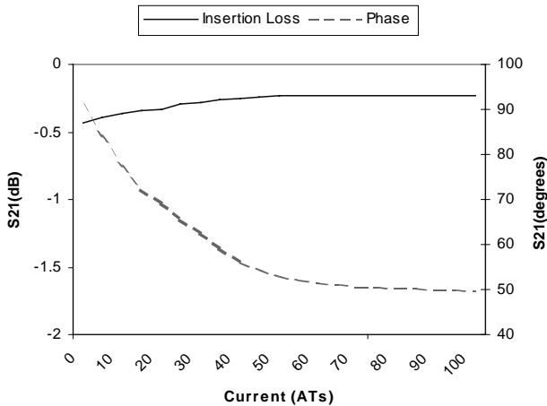
Figure 6. Measured phase shift and insertion loss vs. bias current.
