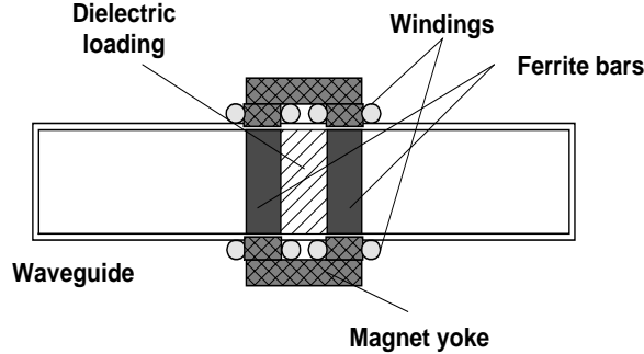
Figure 2. Cross section of a waveguide phase shifter.
