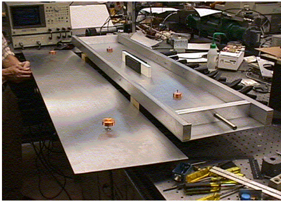
Figure 4. 2" height waveguide loaded with YIG and alumina slabs, and two coax-to-waveguide transitions.
