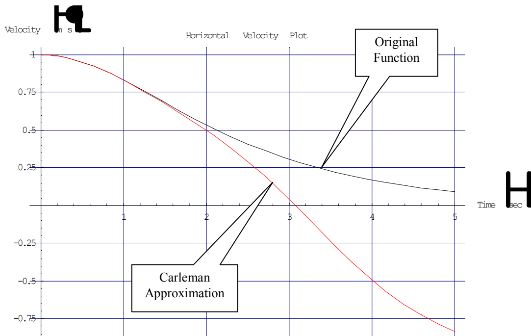
Figure 13 The original horizontal velocity function compared with the Carleman linearization technique over a time interval of 5 seconds using fourth order polynomials yielding a system of 30 ODEs
