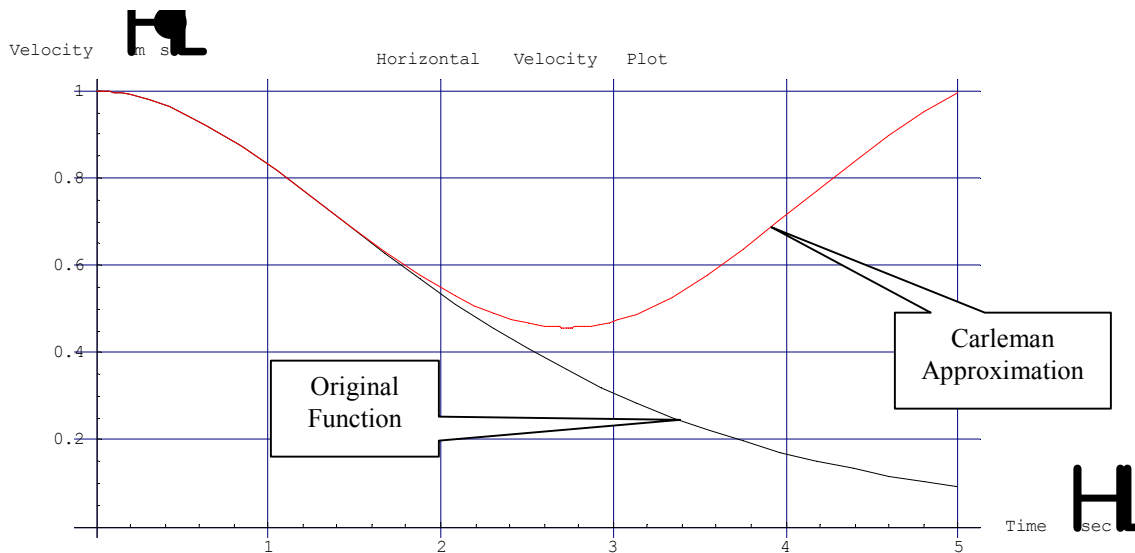
Figure 15 The original horizontal velocity function compared with the Carleman linearization technique over a time interval of 5 seconds using fifth order polynomials yielding a system of 62 ODEs
