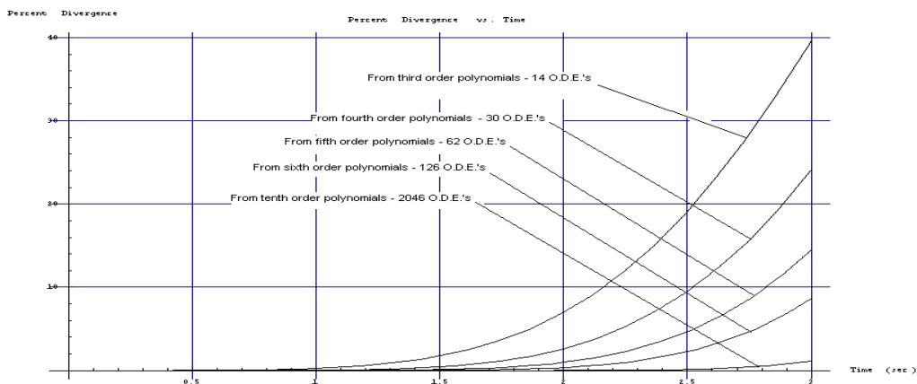
Figure 30 Percent divergence versus time for varying levels of matrix complexity for the ballistic trajectory problem
