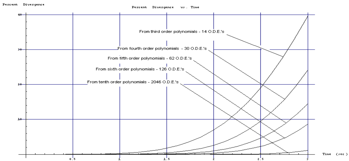
Figure 21 Percent divergence versus time for varying levels of matrix complexity
