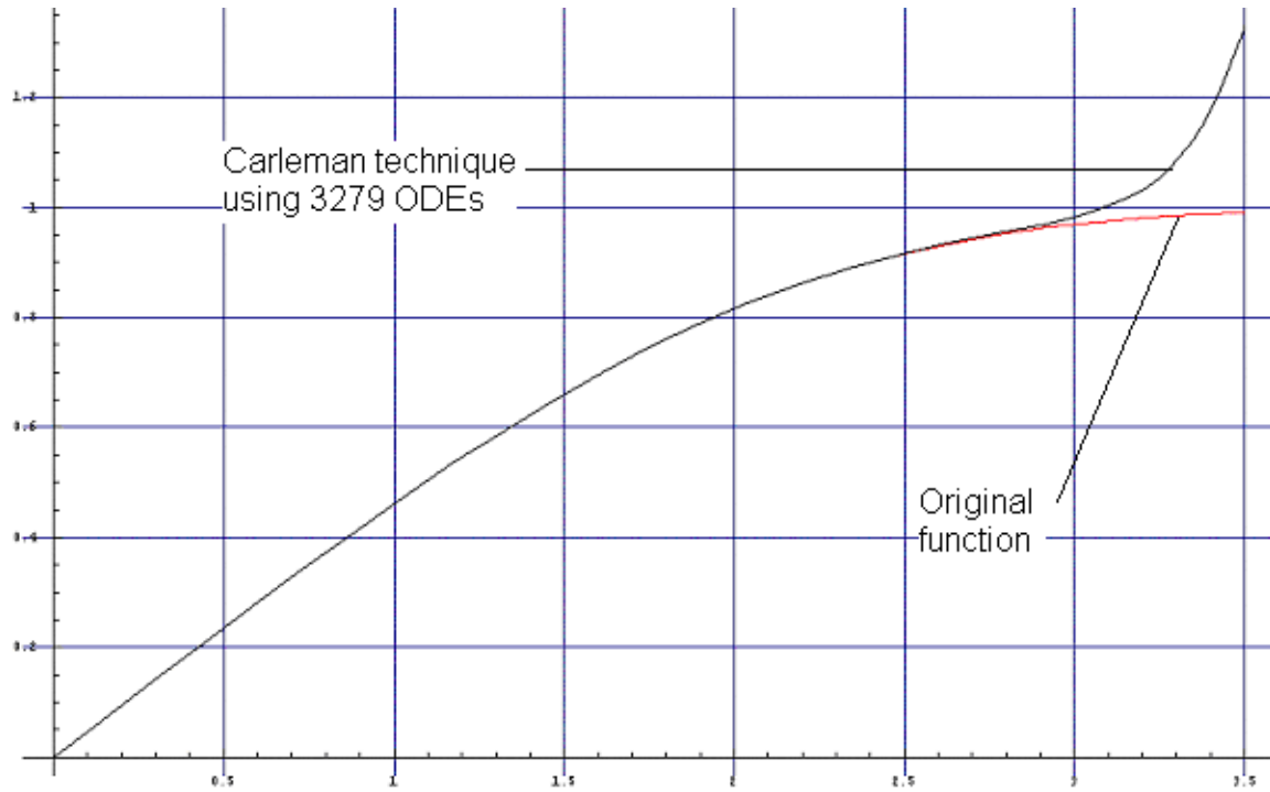
Figure 32 Convergence of the Carleman technique for the boundary layer problem
