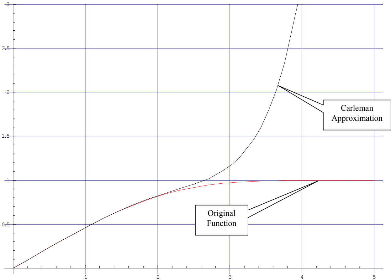
Figure 23 The original boundary layer function compared with the Carleman linearization technique over a time interval of 5 seconds using sixth order polynomials yielding a system of 1092 ODEs
