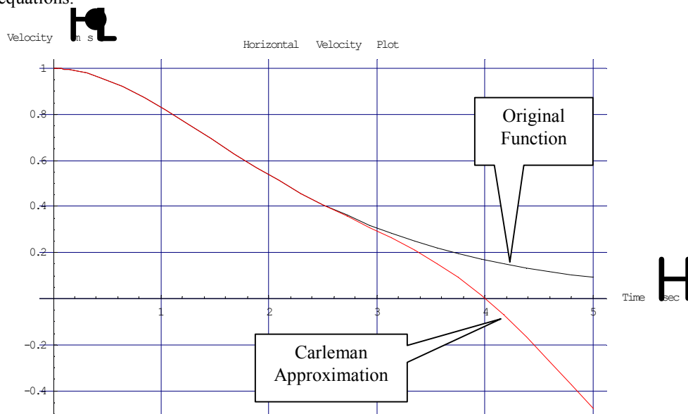
Figure 19 The original horizontal velocity function compared with the Carleman linearization technique over a time interval of 5 seconds using tenth order polynomials yielding a system of 2046 ODEs
