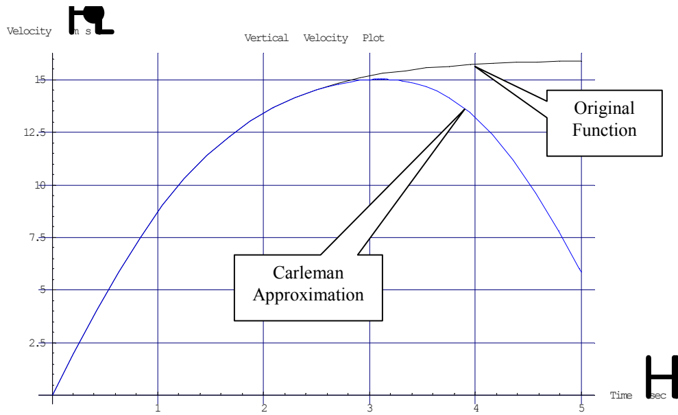
Figure 20 The original vertical velocity function compared with the Carleman linearization technique over a time interval of 5 seconds using tenth order polynomials yielding a system of 2046 ODEs
