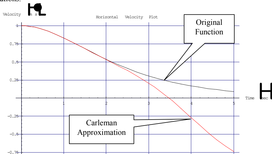
Figure 17 The original horizontal velocity function compared with the Carleman linearization technique over a time interval of 5 seconds using sixth order polynomials yielding a system of 126 ODEs
