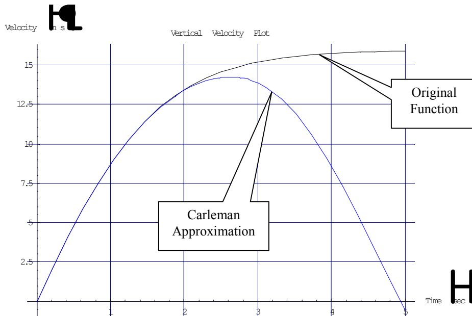
Figure 18 The original vertical velocity function compared with the Carleman linearization technique over a time interval of 5 seconds using sixth order polynomials yielding a system of 126 ODEs
