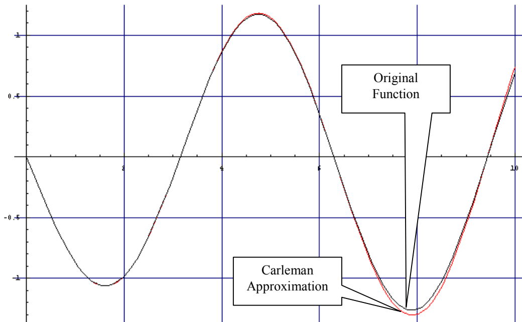
Figure 26 Van der Pol's equation compared with the Carleman linearization technique over a time interval of 10 seconds \varepsilon = 0.1
