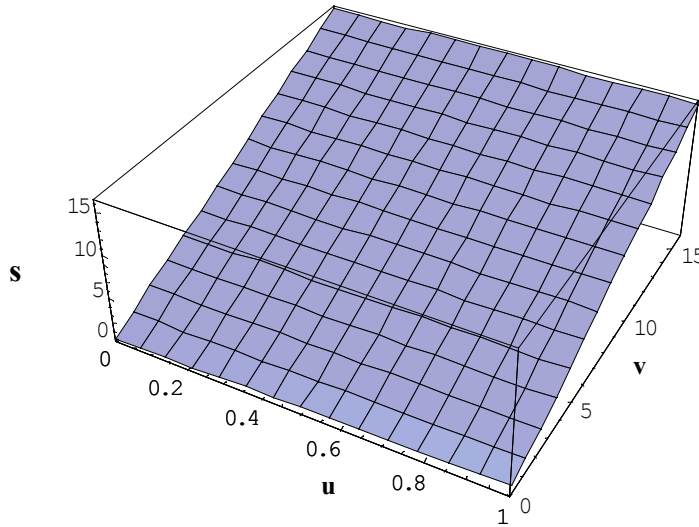
Figure 7 Surface plot representing the speed vector
