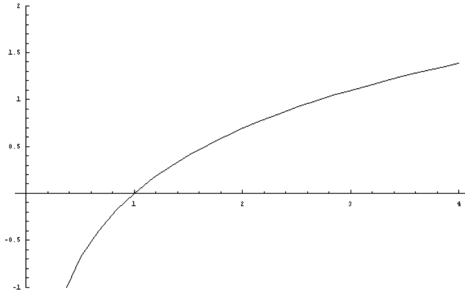
Figure 27 Plot of \text{Log}[x] for x = 0 to 3
