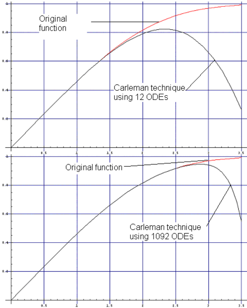
Figure 31 Convergence of the Carleman technique for the boundary layer problem
