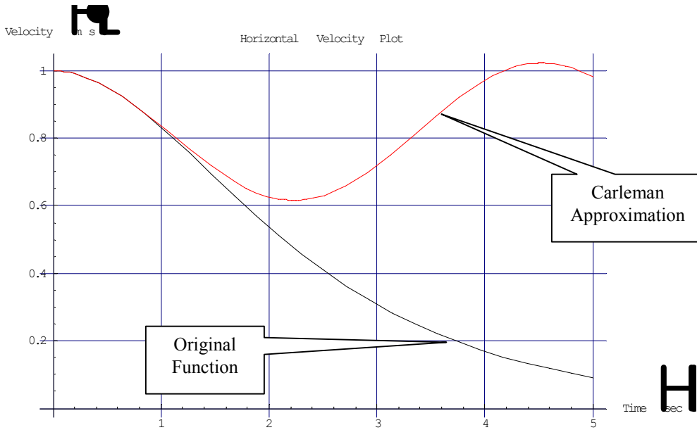
Figure 11 The original horizontal velocity function compared with the Carleman linearization technique over a time interval of 5 seconds using third order polynomials yielding a system of 14 ODEs
