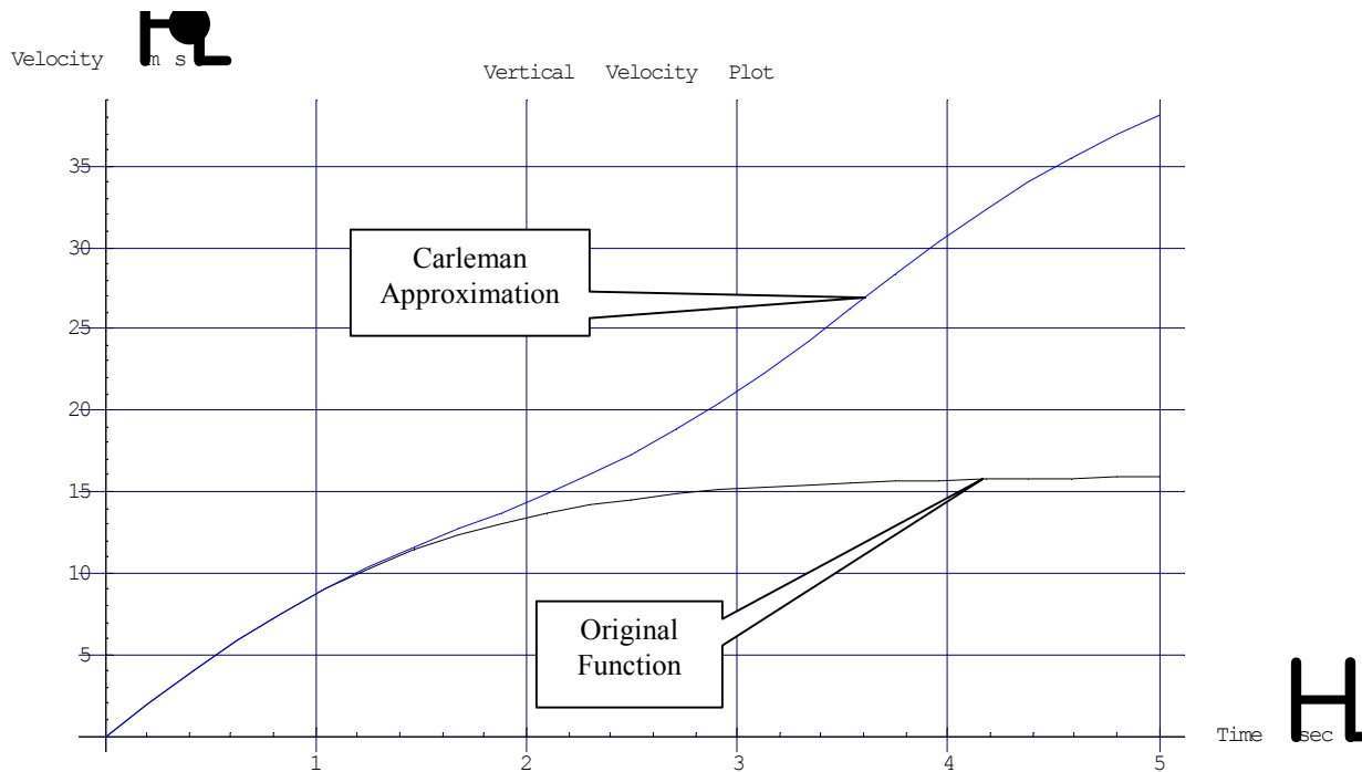
Figure 12 The original vertical velocity function compared with the Carleman linearization technique over a time interval of 5 seconds using third order polynomials yielding a system of 14 ODEs
