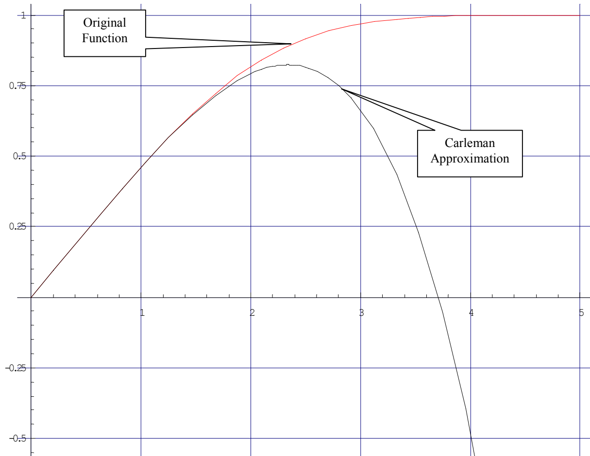
Figure 22 The original boundary layer function compared with the Carleman linearization technique over a time interval of 5 seconds using quadratic polynomials yielding a system of 12 ODEs
