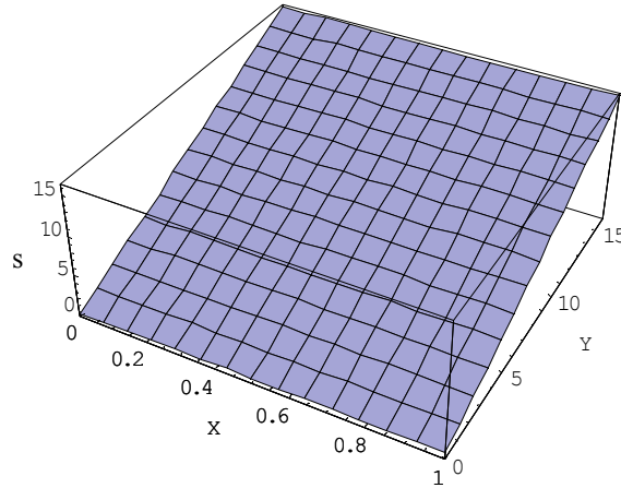
Figure 8 Surface plot of approximation of speed that converts \sqrt{u^2 + v^2} into a polynomial
