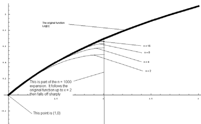
Figure 28 Plot of Taylor series expansion approximations for different “n” number of terms in the Taylor series expansion compared to the original function \text{Log}[x]
