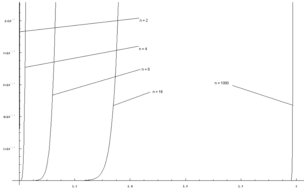
Fig. 29 Shows how much the Taylor series expansion diverges from the function \text{Log}[x] as x increases for “ n ” number of terms in the Taylor series expansion
