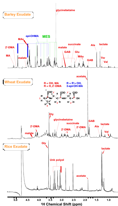
Figure 1. 1 H NMR spectra of whole root exudates from barley, wheat, and rice under a combined Fe deficient and Cd treatment. GAB, \gamma -amino-butyrate; MES, morpholino-ethanesulfonate; epi -OHMA, epi -hydroxy mugineic acid; 2'-DMA, 2'-deoxy-mugineic acid; Unk polyol, unknown polyol.
