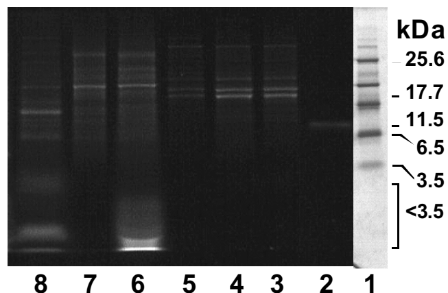
Figure 2. SDS-PAGE of bromobimane-tagged SH-rich peptides and proteins from wheat, rice, and clam tissues. Lanes 1, MW standards; 2, rabbit metallothionein (MT); 3-5, clam MT extracts; 6,7, Cd-treated and control wheat root extracts; 8, Cd-treated rice shoots, respectively.
