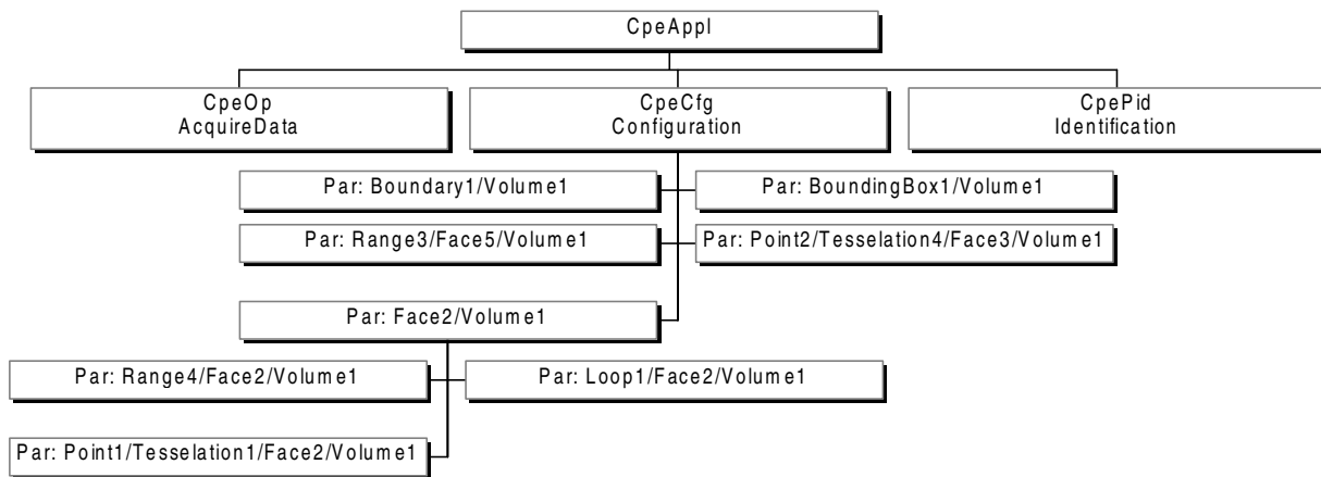
Figure 4: Example configuration of PIA/CAD/CAPRI application wrapper
