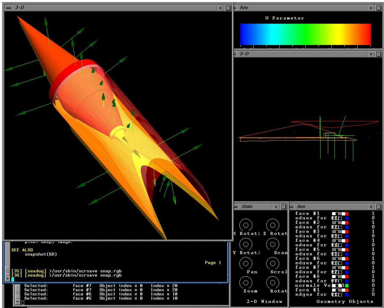
Figure 5: RBCC propulsion system as displayed by CAPRI
