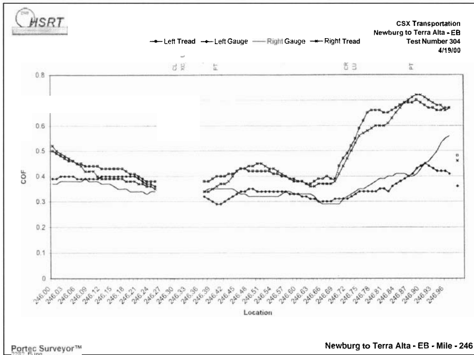
Figure 11. Rail Friction near MP 246 — Baseline Period
