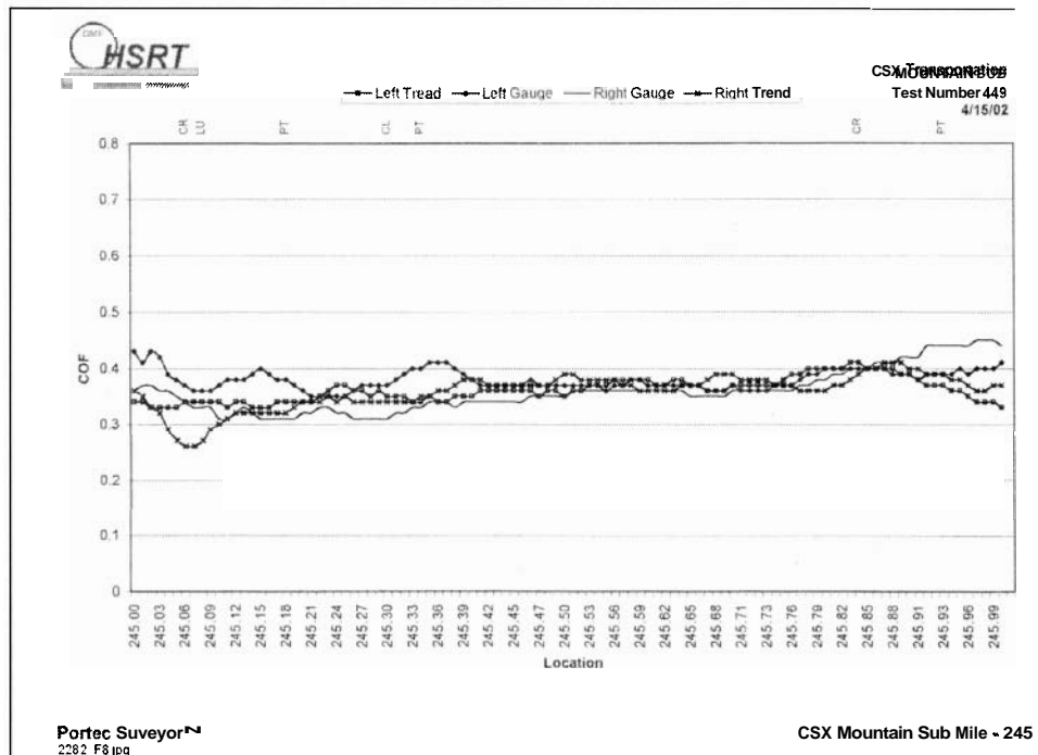
Figure 14. Rail Friction near MP 245 — During TOR Implementation Period
