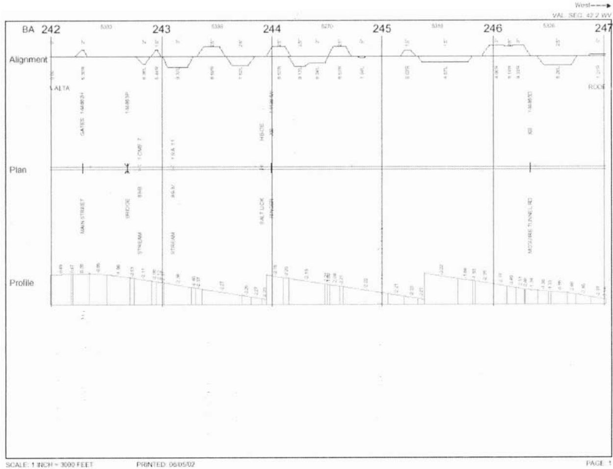
Figure 4a. Track Chart MP 242 to 247
