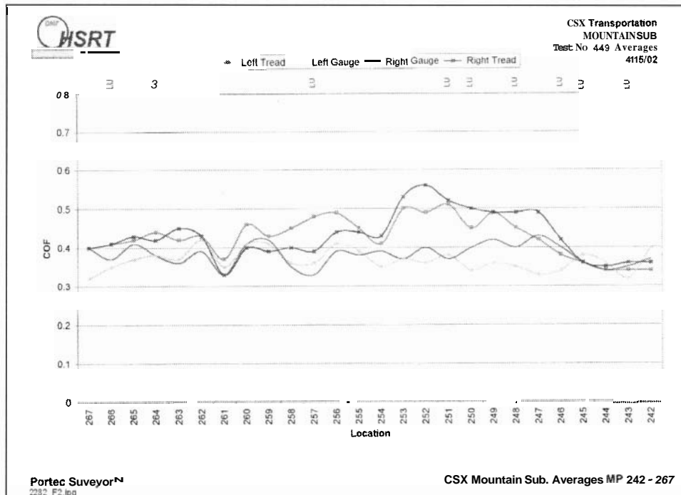
Figure 8. Rail Friction Map of 25 Miles - During TOR Implementation, April 2002
