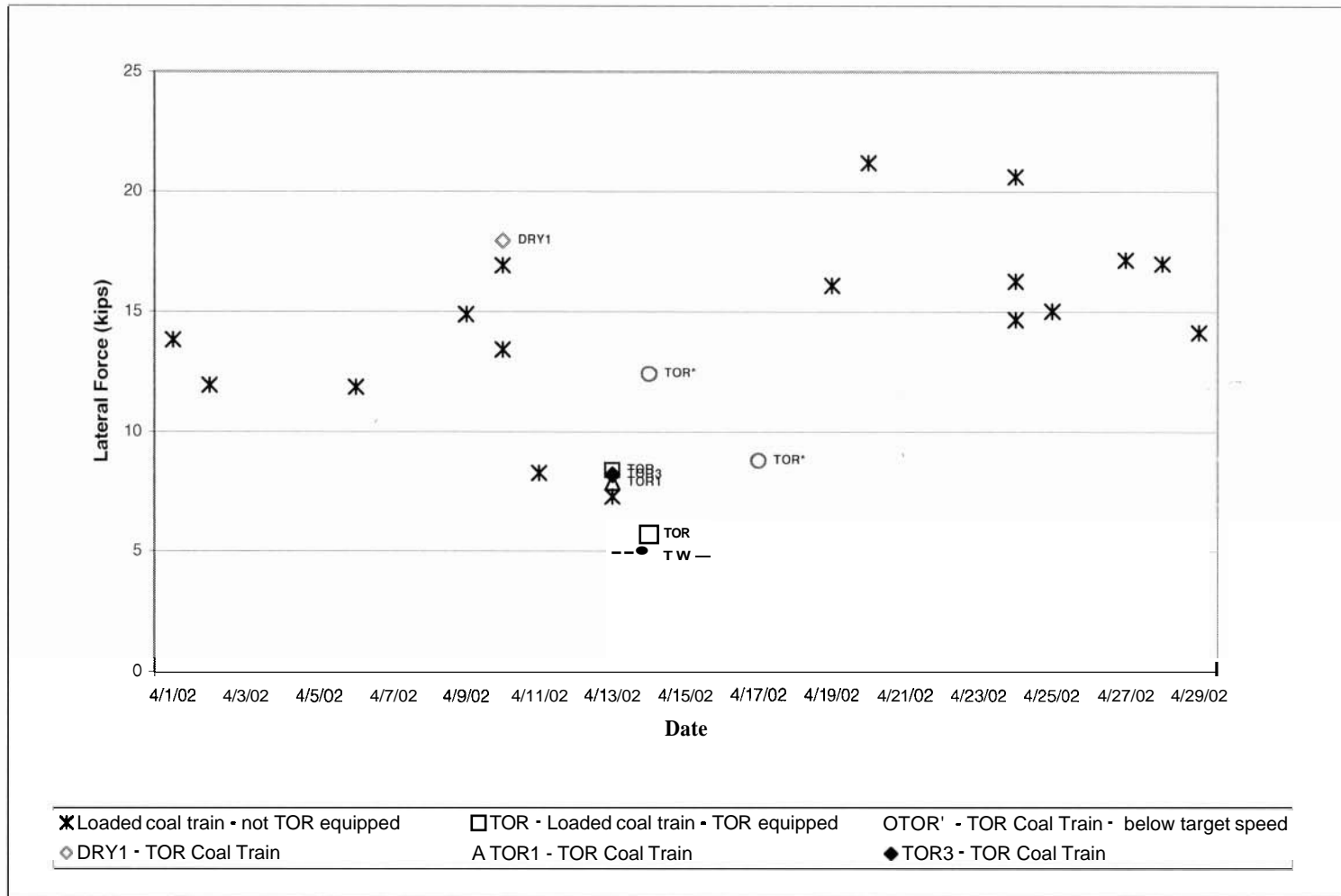
Figure 17b. Detailed Low Rail Lateral Force Performance During TOR Implementation Stage — April 2002
