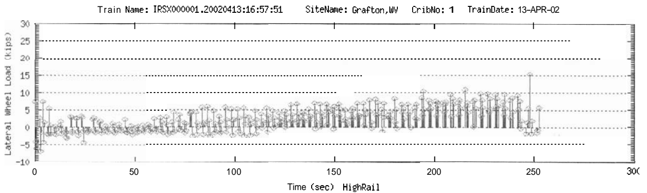
Figure 22. High Rail Lateral Force History of Third TOR-Equipped Train During TOR Implementation Period — Train Pass at 5:00 p.m. on April 13,2002
