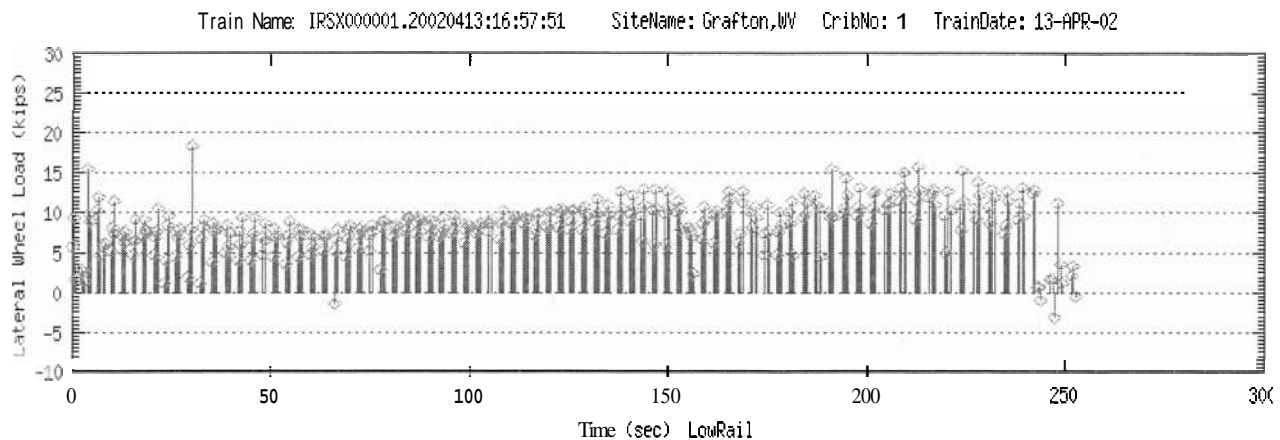
Figure 23. Low Rail Lateral Force History of Third TOR-Equipped Train During TOR Implementation Period — Train Pass at 5:00 p.m. on April 13,2002
