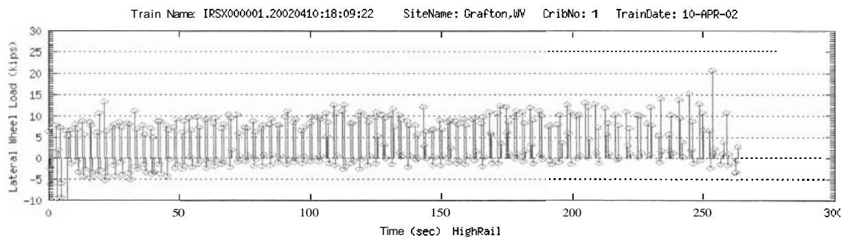
Figure 18. High Rail Lateral Force History of One Train During Baseline Period — Train Pass at 6:09 p.m. on April 10,2002
