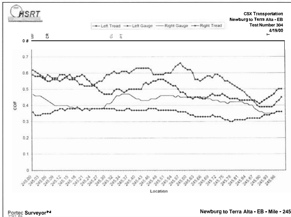
Figure 12. Rail Friction near MP 245 — Baseline Period
