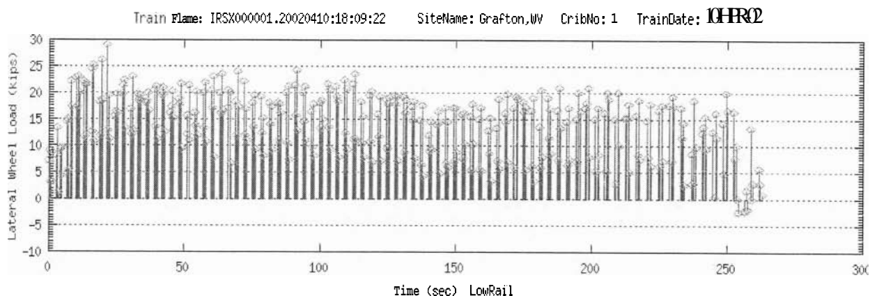
Figure 19. Low Rail Lateral Force History of One Train During Baseline Period — Train Pass at 6:09 p.m. on April 10,2002
