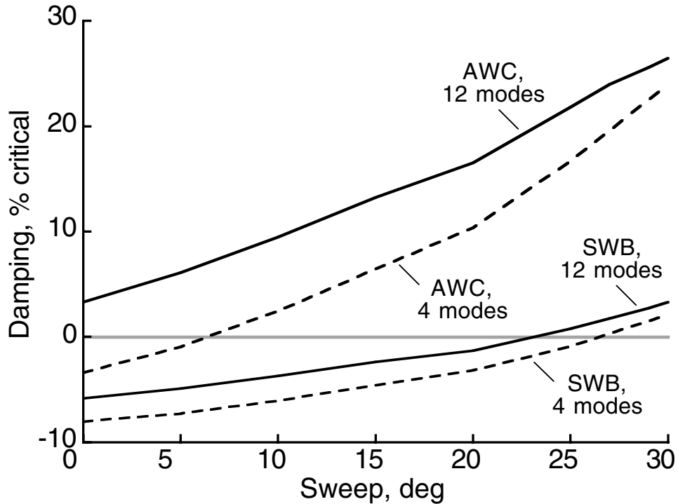
Figure 23. Effects of simplified dynamic model on the most sensitive modes, for sweep with inboard tuning mass at 300 knots with -30 deg \delta_3 .
