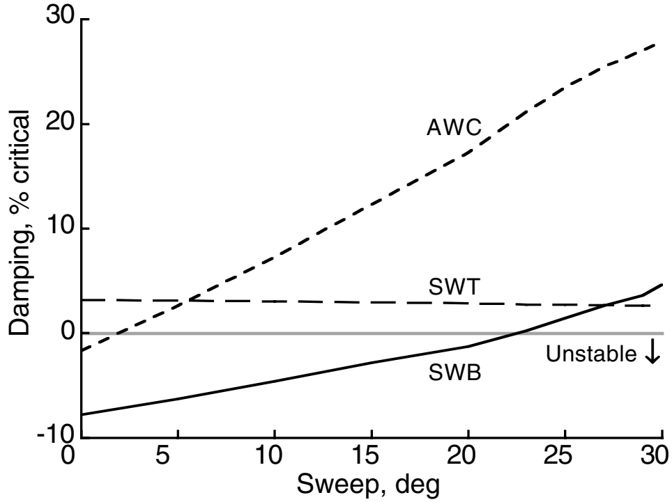
Figure 14. Variation of damping with combined sweep and tip-mass offset at 300 knots with -30 \text{ deg } \delta_3 . Offset is calculated as equivalent sweep (see fig. 11(e)).
