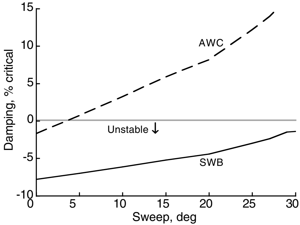
Figure 15. Variation of damping with sweep and fixed tip-mass position at 300 knots with -30 \text{ deg } \delta_3 . Offset is calculated as equivalent sweep (see fig. 11(d)).
