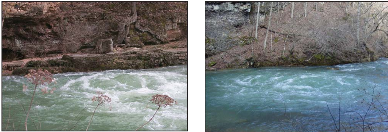
Figure 3. Big Spring (left) and Greer Spring (right), two large springs with recharge areas in the exploration area (photographs courtesy of Brian S. Fredrick, U.S. Geological Survey, 2002).
