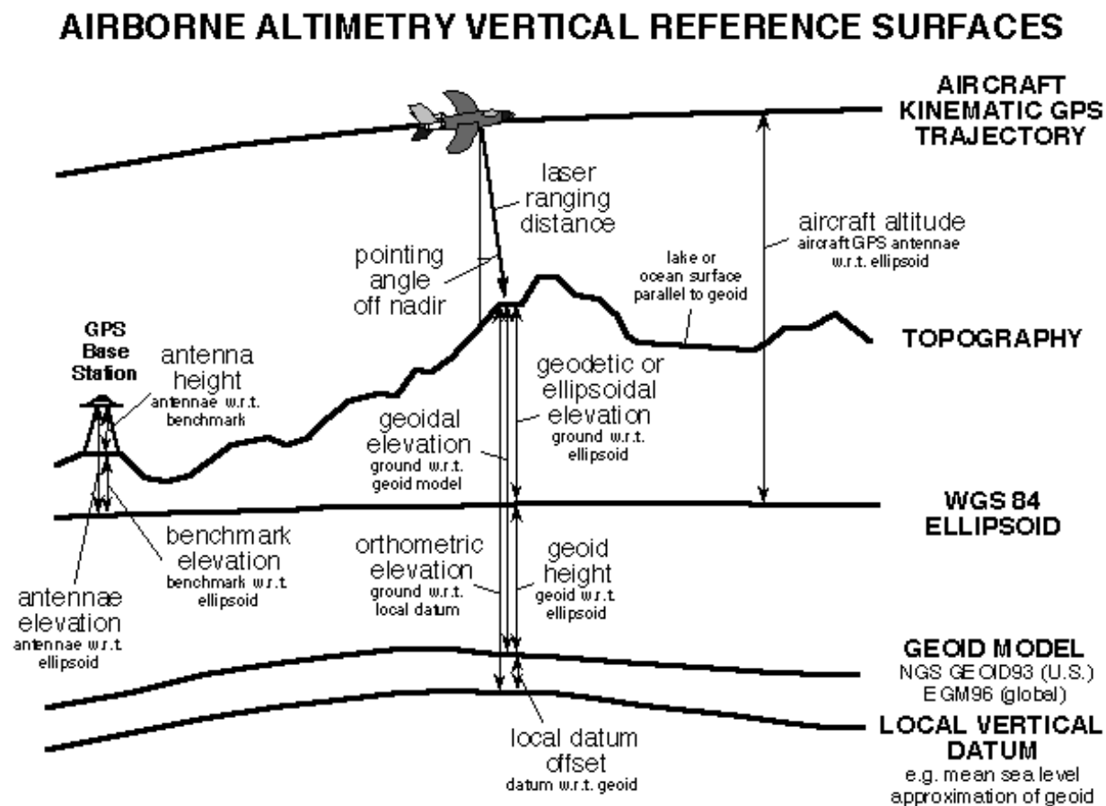
Figure 1: Airborne Altimetry Vertical Reference Surfaces
