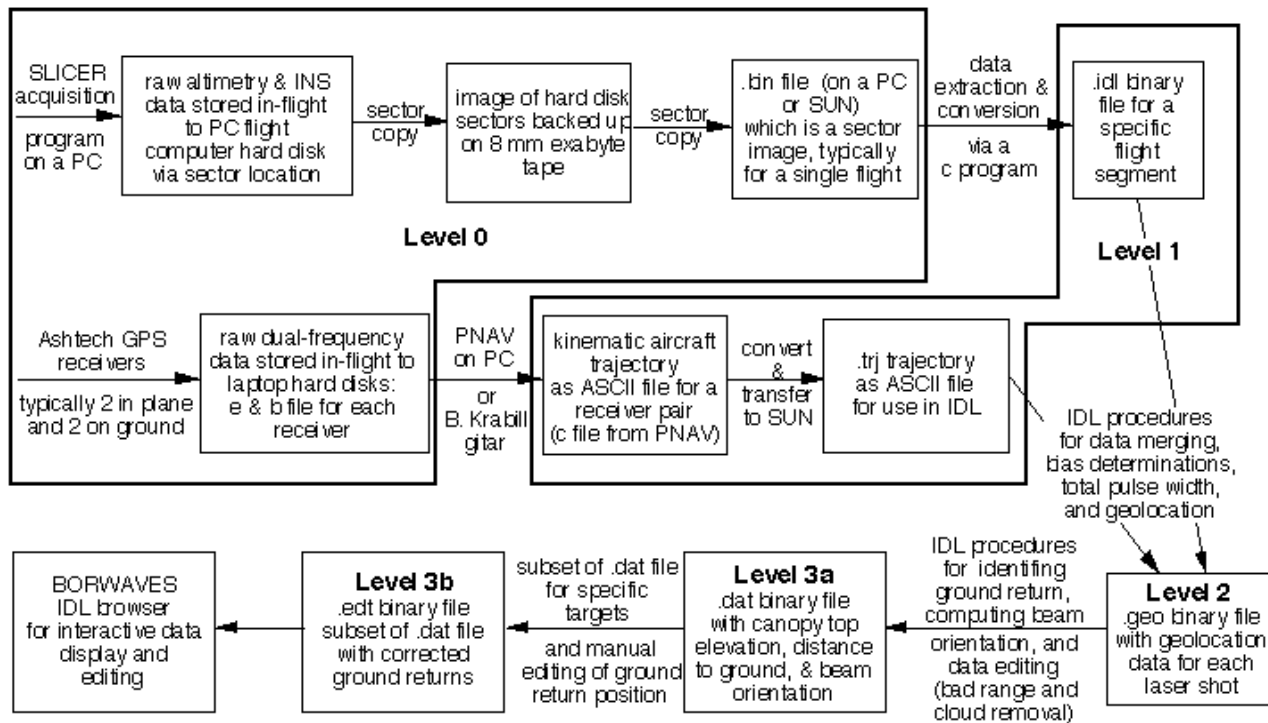
Figure 7: SLICER Data Processing Flow
