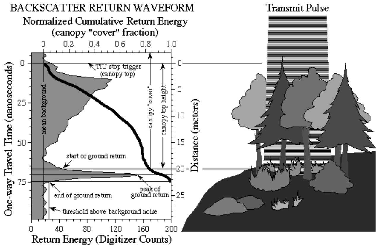
Figure 3: Backscatter Return Waveform
