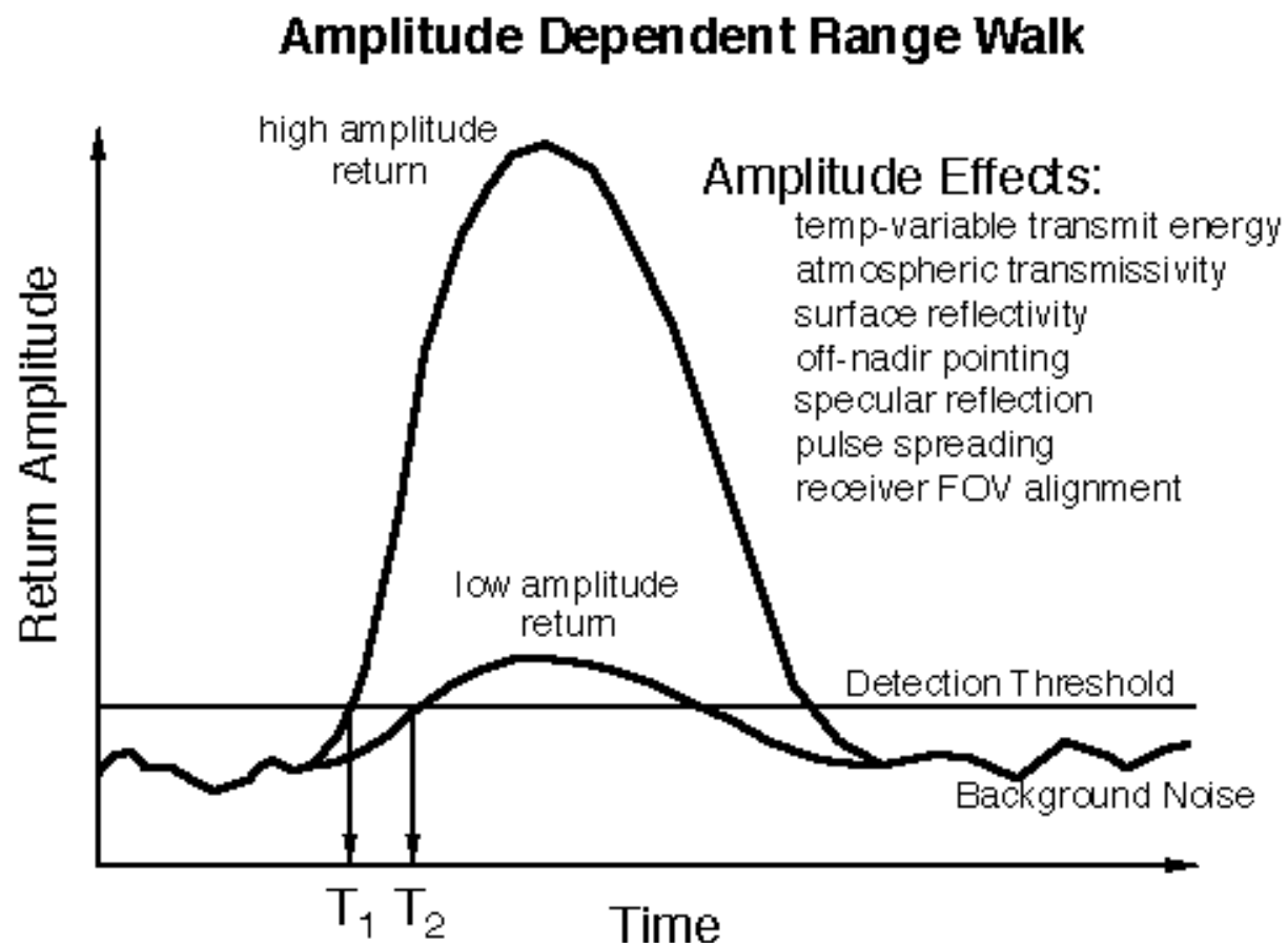
Figure 8: Amplitude Dependent Range Walk
