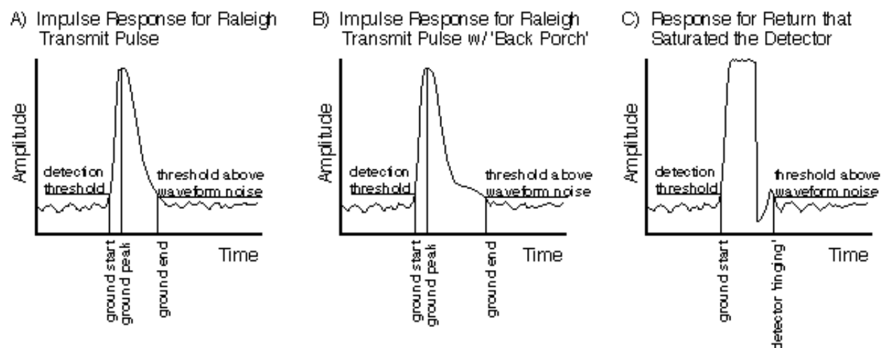
Figure 10: Characteristic Backscatter Waveforms from a Flat, Smooth Surface
