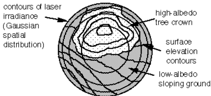
Figure 2: Laser Altimetry Echo Recovery
