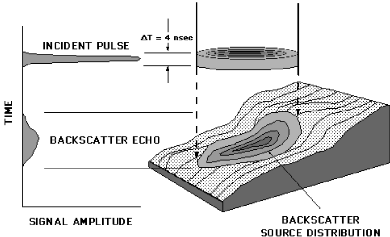
Figure 11: Pulse Spreading Due to Surface Slope and Roughness
