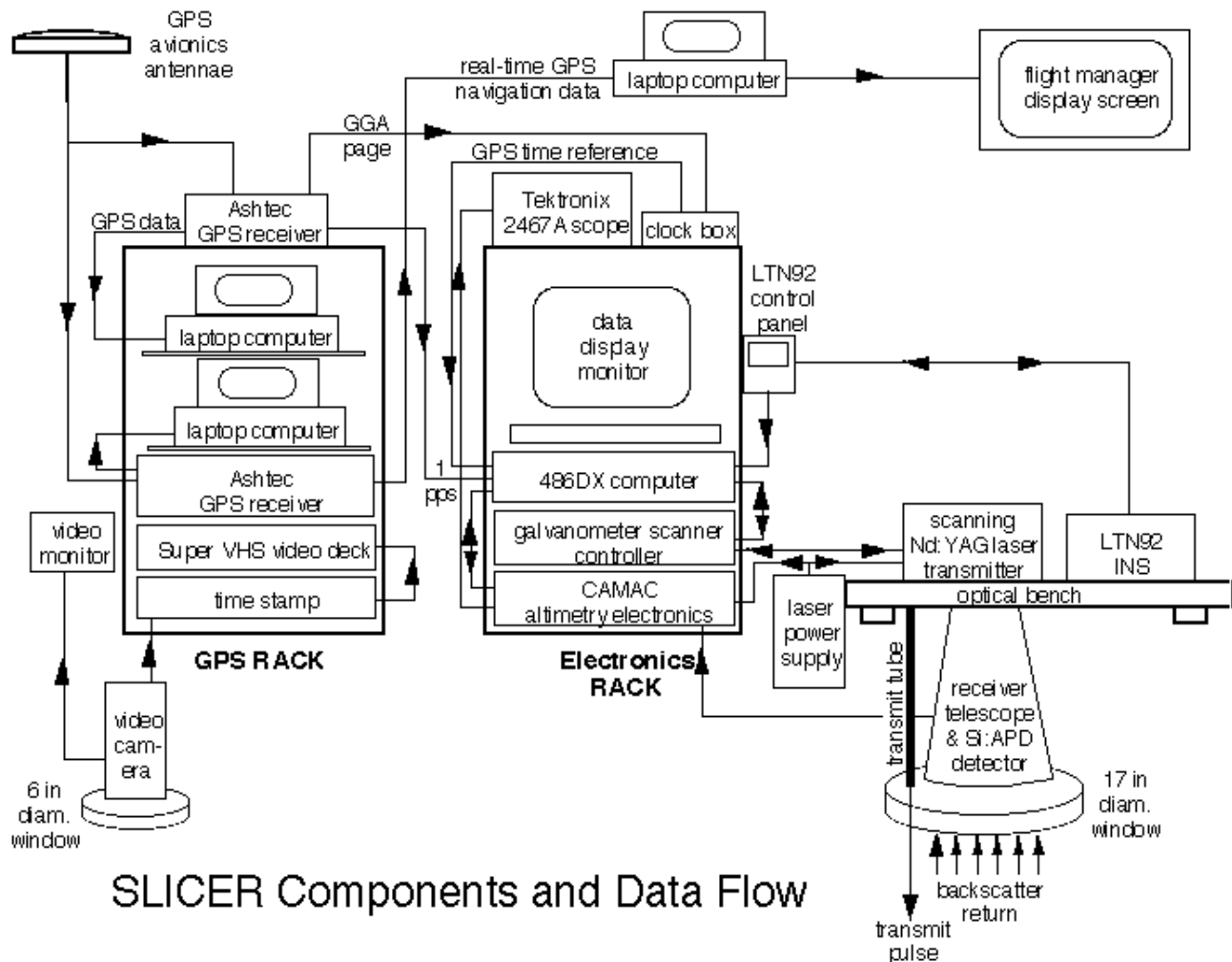
Figure 5: SLICER Components and Data Flow
